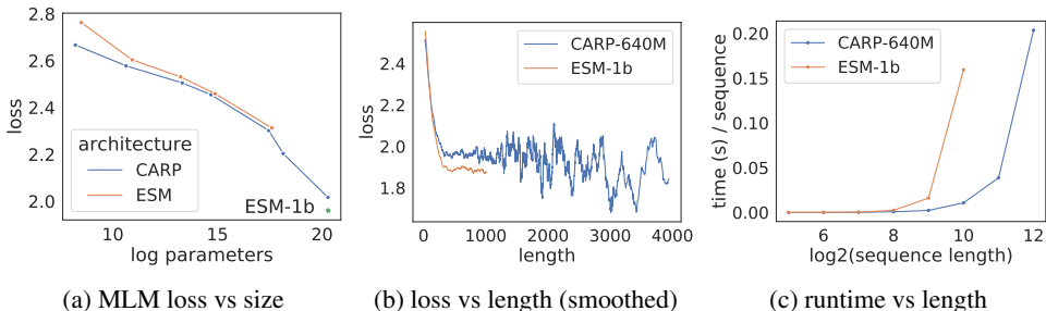
Figure 2: Comparisons between CARP and the ESM-1b transformer.
