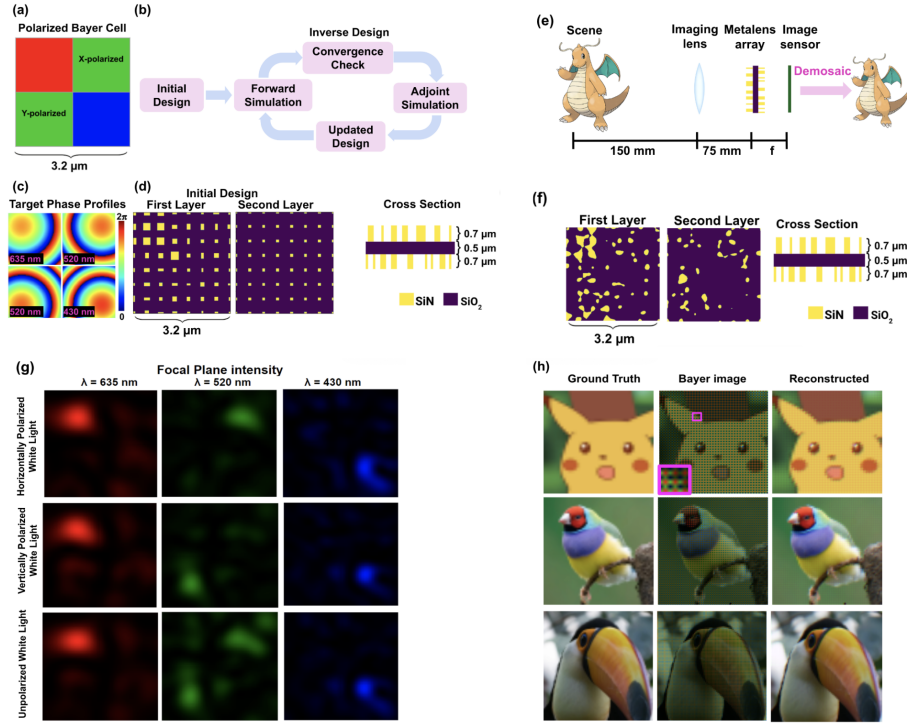
Fig. 1. (a) Target Bayer cell: incident light is sorted and focused into four color-specific pixels, with the two green pixels focusing horizontally and vertically polarized light. (b) Inverse design flowchart. (c) Target phase profiles for red, green, and blue. (d) Initial design and its cross-section view. (e) Color imaging experimental Setup. (f) Optimized Bayer cell structure. (g) Focal plane intensity at 635 nm, 520 nm, and 430 nm for a pixel illuminated by horizontally polarized, vertically polarized, and unpolarized white light. (h) Full-color imaging: the left column shows ground truth images, the middle shows RRGB Bayer images by spectral response, and the right shows reconstructed images.
