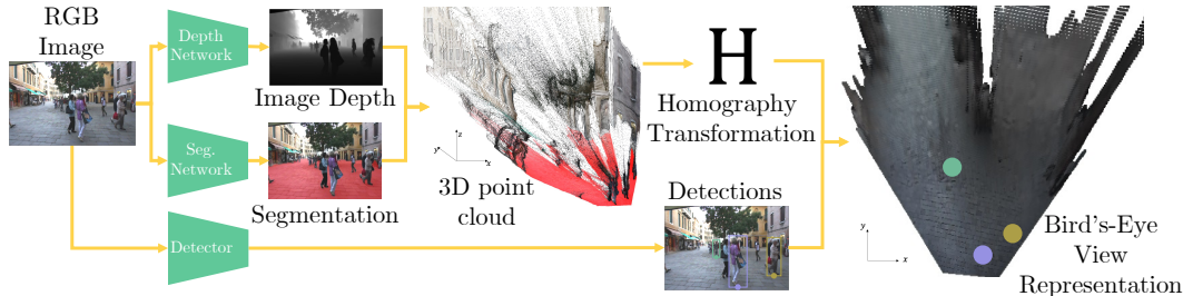
Figure 3: We estimate the homography H for a sequence by reconstructing a 3D point cloud using a monocular depth estimator. We obtain ground image-to-point-cloud correspondences using a semantic segmentation model that masks ground pixels as needed to estimate the homography matrix. With the estimated homography matrix, we transform the bottom points of bounding boxes to 2D BEV coordinates.
