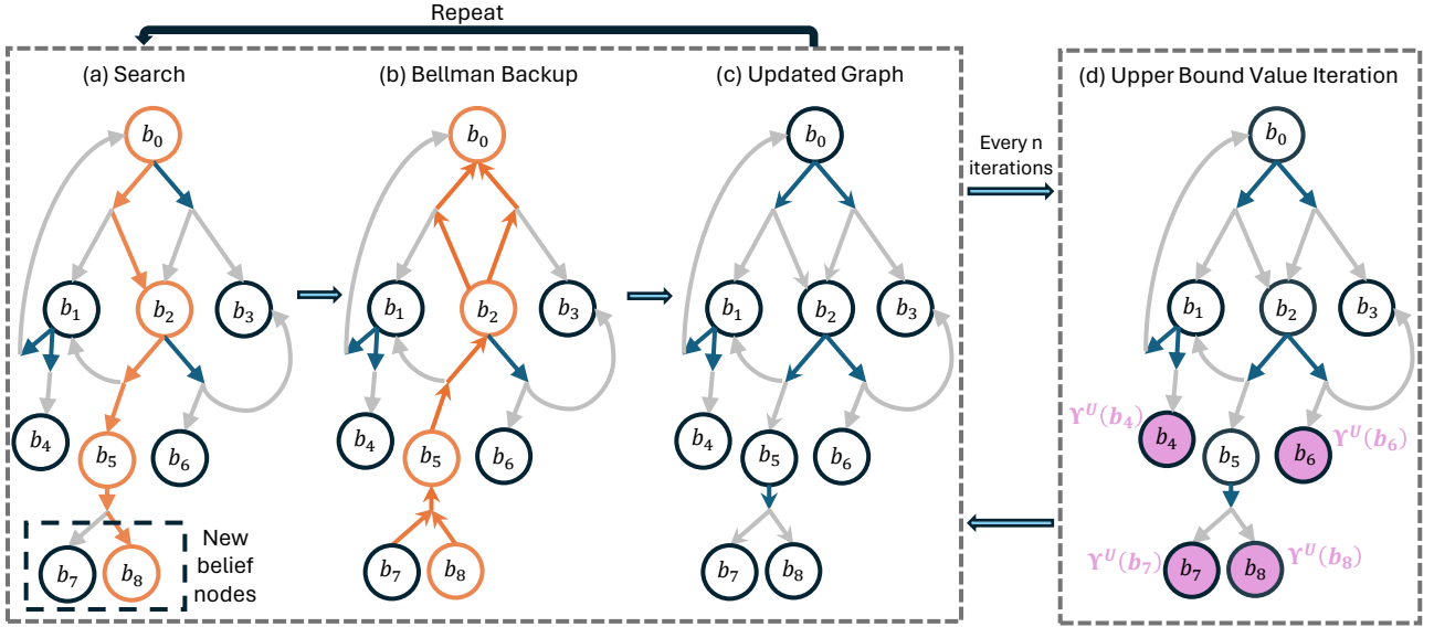
Figure 2: Overview of HSVI-RP. The algorithm incrementally constructs a belief graph using trial-based search, and maintains upper and lower bound values for each belief node. In each trial, actions and observations are selected using a heuristic based on the upper and lower bound values to visit a sequence of belief nodes (orange). After each trial, value bounds for each visited node are updated using local Bellman backups. Every n iterations, upper bound values for all nodes are reset, and frontier nodes (purple) are re-initialized using the upper bound value set \Upsilon^U , and value iteration is performed. This allows better improvement of upper bound values for MRPP.
