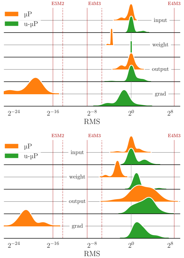
Figure 4. Per-tensor \text{RMS} = \sqrt{\sigma^2 + \mu^2} across u- \mu P and \mu P models at initialization (top) and after training (bottom). u- \mu P tensors have RMS that starts close to 1 and remains within E4M3 range at the end of training. Dashed and solid red lines show each format’s min. normal and subnormal values.
