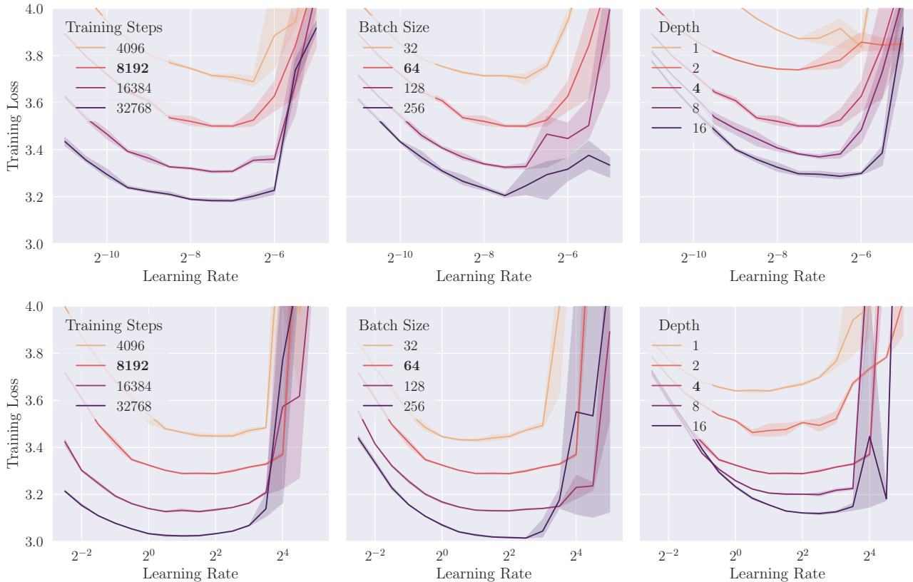
Figure 5. Learning rate transfer for \mu P (top) and u- \mu P (bottom), over training steps, batch size and depth. See Figure 1 (top) for transfer over width. The default shape parameter for other panels is shown in bold. The shaded area shows the 95% confidence interval for the mean.
