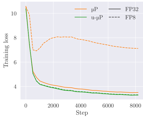
Figure 8. FP8 training by direct cast, width 256, default hyperparameters, \eta = (2^1, 2^{-8}) for (u- \mu P, \mu P).
