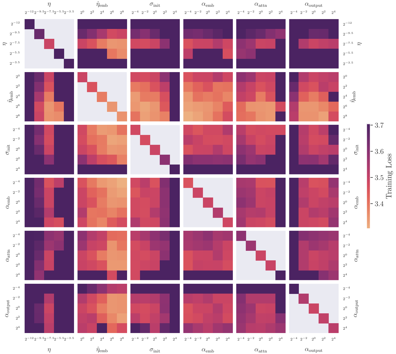
Figure 11. Hyperparameter coupling sweep for \mu P. Note strong coupling between optima, e.g. in the cases of (\hat{\eta}_{emb}, \sigma_{init}) and (\eta, \alpha_{attn}) . See also: u- \mu P, Figure 12. Across all grids, the average training loss degradation from using the optimum from the wrong row/column is 0.08, which is worse than u- \mu P (0.03).
