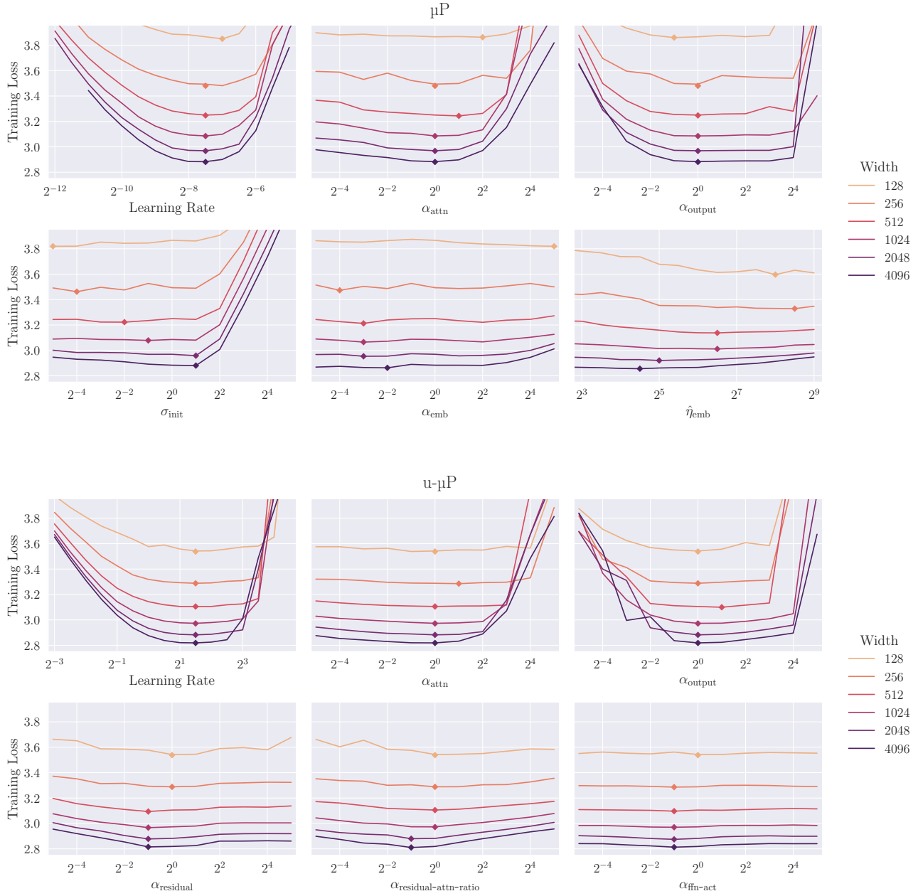
Figure 7. Transfer of model hyperparameters over width for \mu P (top) and u- \mu P (bottom). When one hyperparameter is being swept, all others are fixed at 1, with the exception of Learning Rate \eta = (2^{1.5}, 2^{-7.5}) for (u- \mu P, \mu P).
