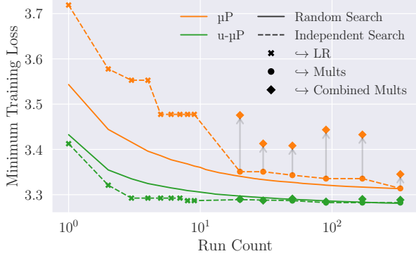
Figure 3. A comparison of random versus independent HP search strategies on \mu P and u- \mu P, showing that u- \mu P parameters are more amenable to independent search, and that combining the results of independent searches of \mu P mults harms performance.
