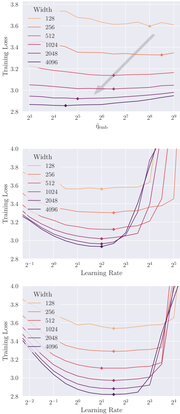
Figure 2. (Top) Transfer of the input LR multiplier over width when using \mu P.
