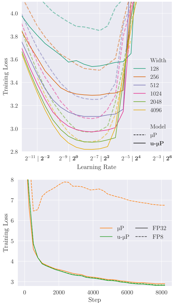
Figure 1. (Top) Using default HPs, u- \mu P models have lower losses and wider basins than \mu P models, while still transferring the optimal learning rate across width.
