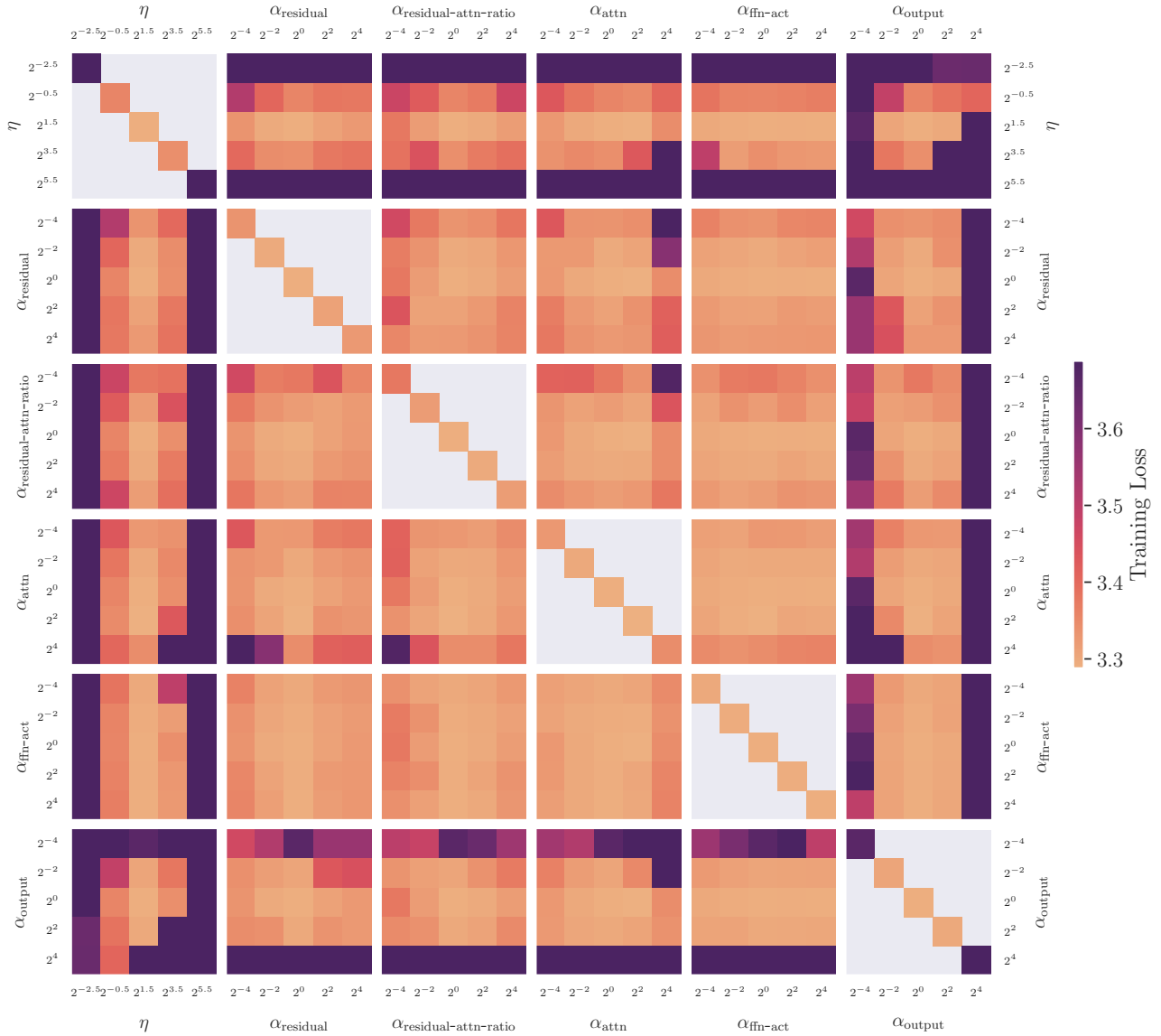
Figure 12. Hyperparameter coupling sweep for u- \mu P. Note less coupling than with \mu P, see Figure 11. Across all grids, the average training loss degradation from using the optimum from the wrong row/column is 0.03, which is better than \mu P (0.08).
