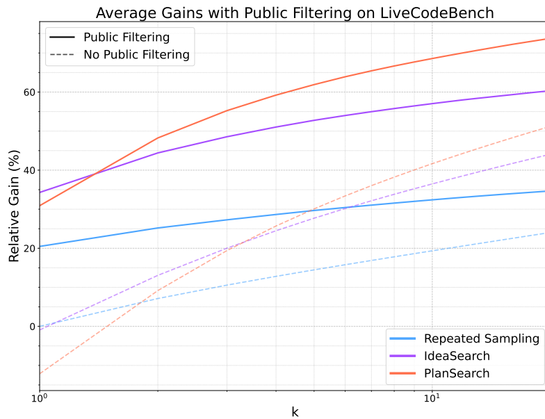
Figure 16: Average performance gain over all models of methods with public test filtering compared to REPEATED SAMPLING@1, plotted over k \in \{1, \dots, 20\} . Note that dotted lines are provided for reference of the base method pass@k (before filtering).
