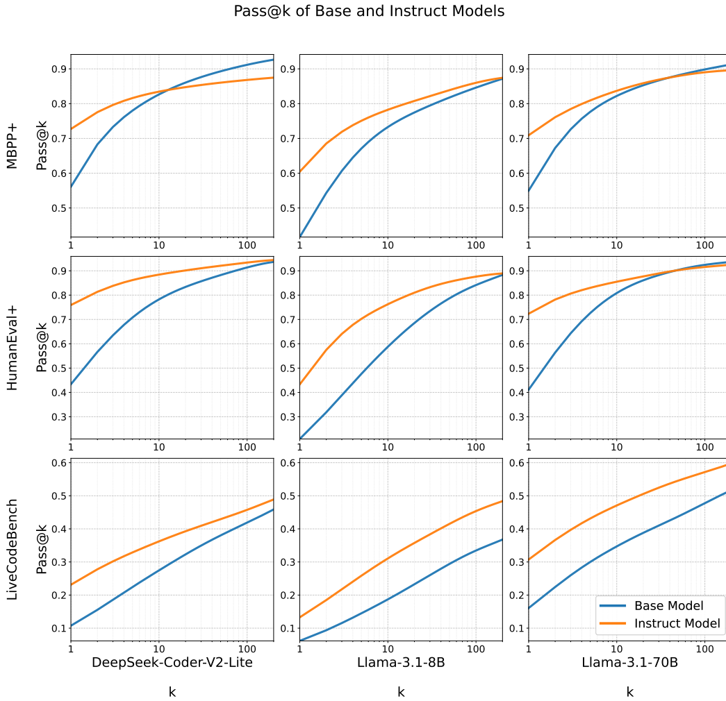
Figure 31: Pass@k curves comparing DeepSeek-Coder-V2-Lite, Llama-3.1-8B, and Llama-3.1-70B base and instruct performance.
