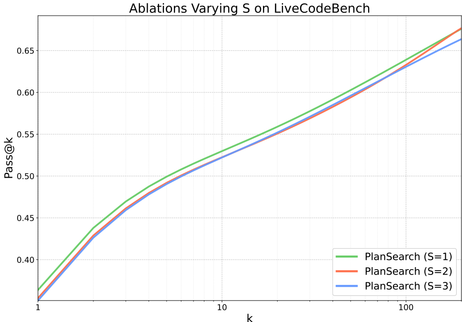
Figure 27: We run ablations of PLANSEARCH with different S —controlling the maximum subset size from a given pool of observations. There is not a large difference between different S , but we find that 1 or 2 is slightly more optimal, although if more completions are desired, S can be increased to 3 as well.
