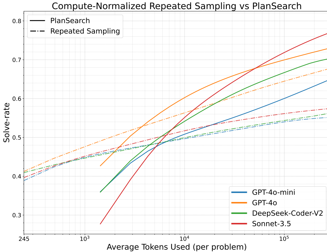
Figure 17: Normalized pass@k by average tokens used per problem. REPEATED SAMPLING uses roughly 244 tokens per completion per problem, and PLANSEARCH uses roughly 1428 tokens per completion per problem. When we normalize compute across methods, we find that PLANSEARCH begins to be more effective than repeated sampling if the user is willing to sample at least 10,000 tokens per problem.
