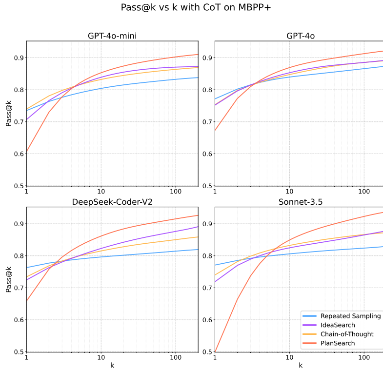
Figure 19: Pass@k graphs on MBPP+, with the Chain-of-Thought baseline.
