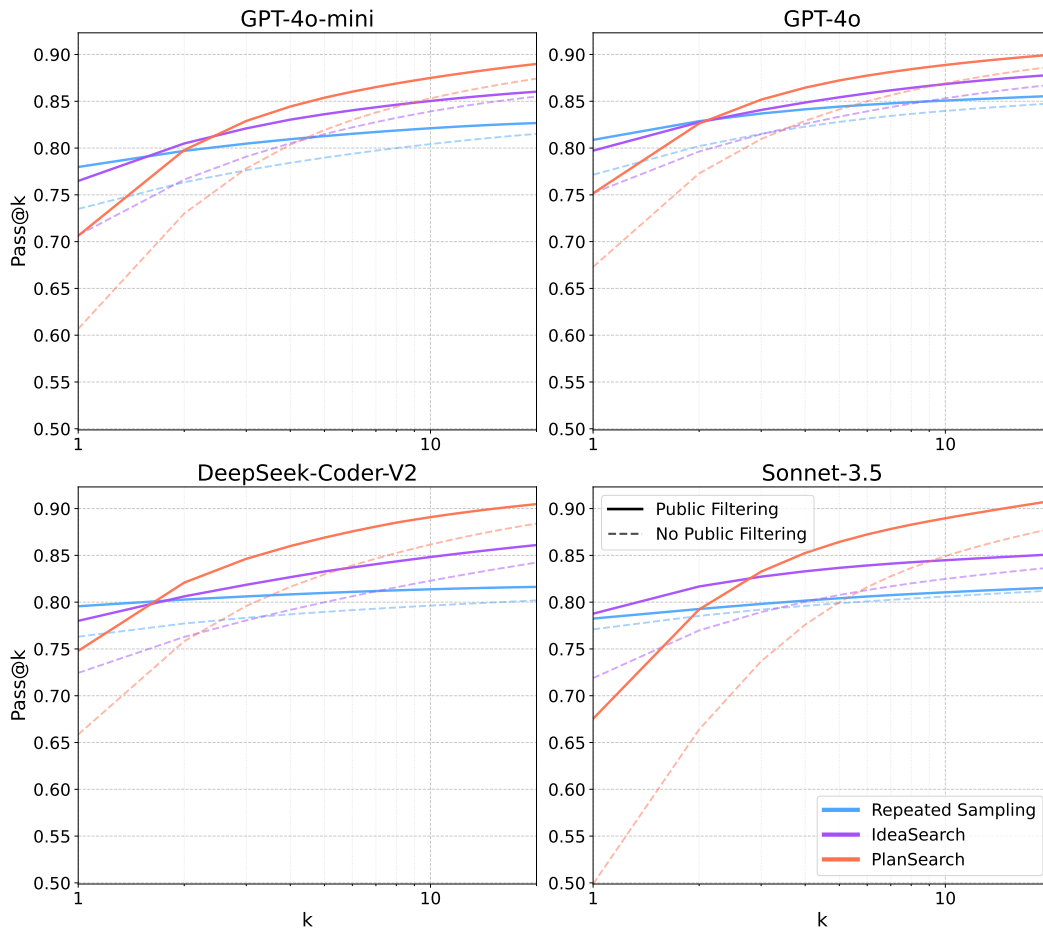
Figure 10: Pass@k performance of all models and methods on MBPP+, with public test filtering, plotted over k \in \{1, \dots, 20\} . Note that dotted lines are provided for reference of the base method pass@k before filtering.
