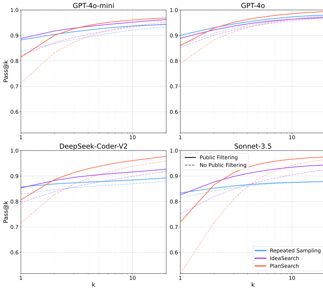
Figure 9: Pass@k performance of all models and methods on HumanEval+, with public test filtering, plotted over k \in \{1, \dots, 20\} . Note that dotted lines are provided for reference of the base method pass@k before filtering.
