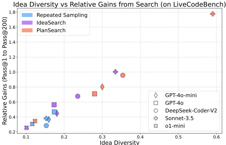
Figure 5: We observe a strong positive correlation between the measured amount of idea diversity (higher score is better) in a search algorithm and the resulting improvements due to search. See Section 6.1 for information regarding the diversity score.
