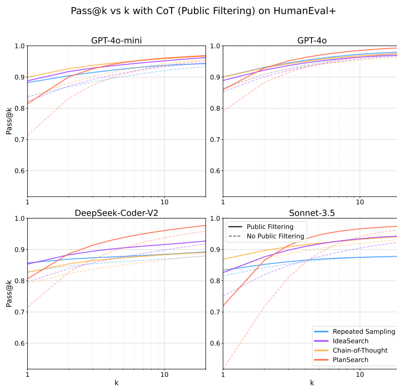
Figure 23: Pass@k graphs on HumanEval+, with the Chain-of-Thought baseline and public filtering.
