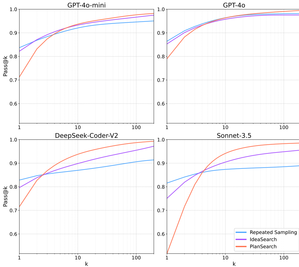
Figure 6: Pass@k performance of all models and methods on HumanEval+, plotted over k \in \{1, \dots, 200\} .
