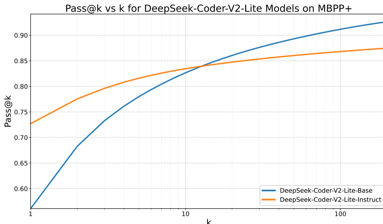
Figure 30: Despite DeepSeek-Coder-V2-Lite-Base having significantly lower pass@1 than its instruct counterpart, we observe that this trend reverses as k increases, suggesting that the instruct model has less diversity than its base model counterpart. We observe this trend for many, but not all, models and benchmarks, and provide the full data in Appendix I.
