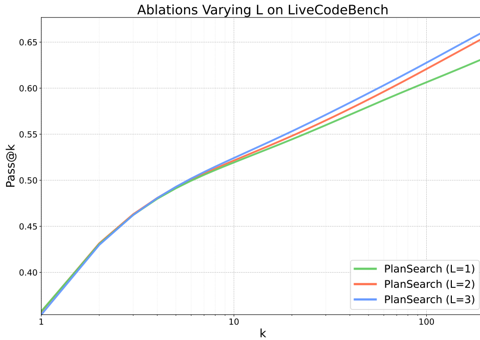
Figure 28: We run ablations of PLANSEARCH with different L —controlling the maximum order of observation used, i.e., how many layers the observation tree will search. We find pass@k scales with respect to increasing L
