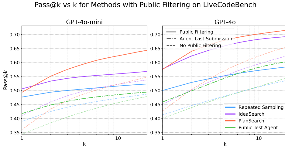
Figure 42: Pass@k curves comparing the basic agentic model’s last submissions only on LiveCodeBench with up to 20 completions and public test filtering.
