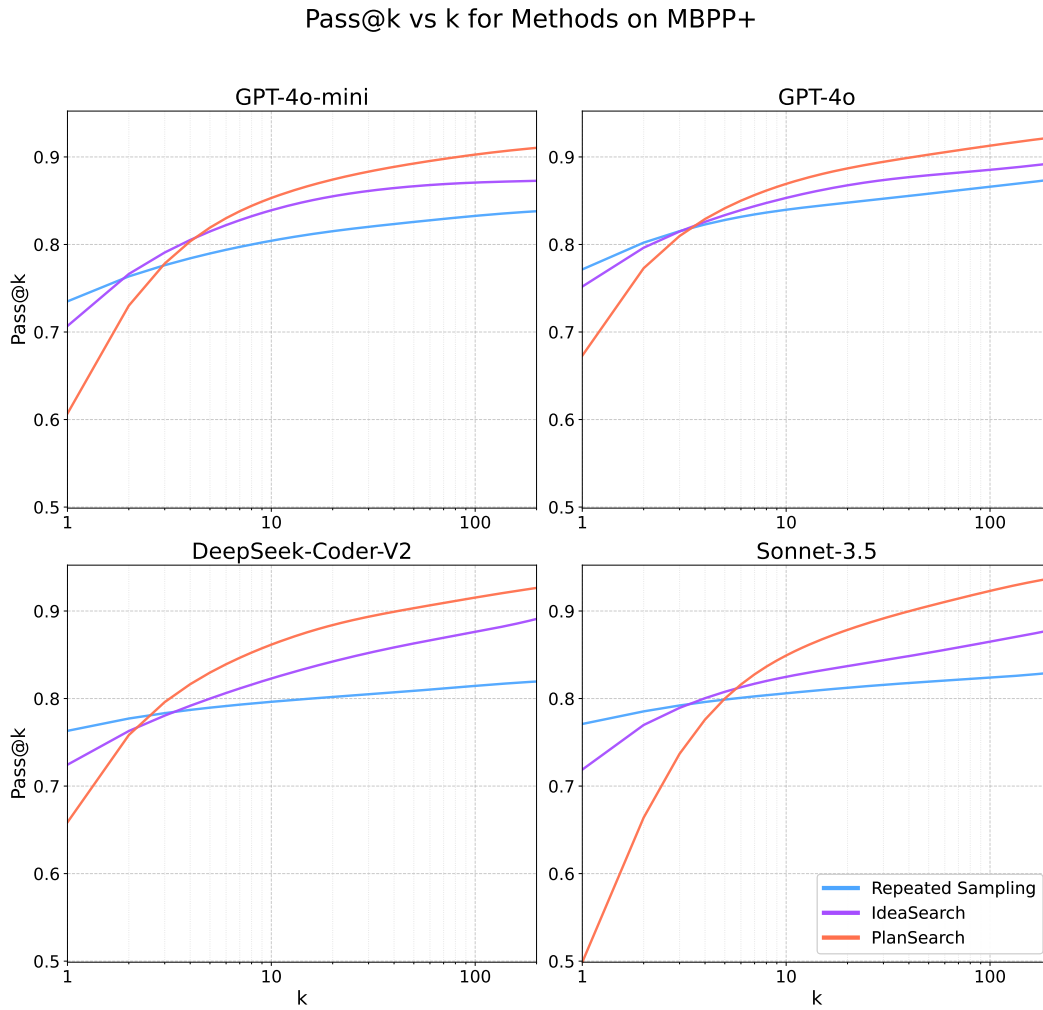
Figure 7: Pass@k performance of all models and methods on MBPP+, plotted over k \in \{1, \dots, 200\} .
