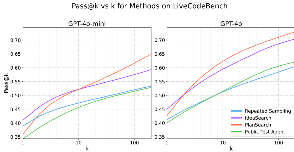
Figure 43: Pass@k curves comparing the basic agentic model with all T generations on LiveCodeBench with up to 200 completions.
