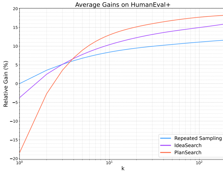
Figure 11: Performance gain over REPEATED SAMPLING@1 averaged over all models on HumanEval+, plotted over k \in \{1, \dots, 200\} .
