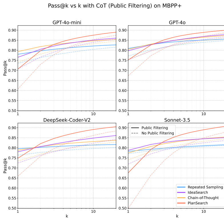
Figure 22: Pass@k graphs on MBPP+, with the Chain-of-Thought baseline and public filtering.
