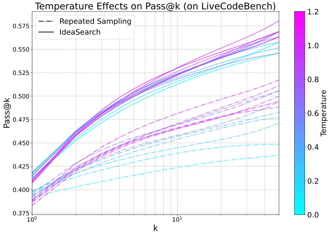
Figure 24: Sweep over temperature in 0.1 increments from 0.0 to 1.2. REPEATED SAMPLING and IDEASEARCH both exhibit pass@k improvements at higher temperature, although it seems that higher temperatures may begin to plateau.
