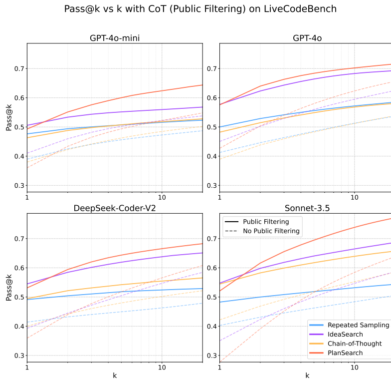
Figure 21: Pass@k graphs on LiveCodeBench, with the Chain-of-Thought baseline and public filtering.
