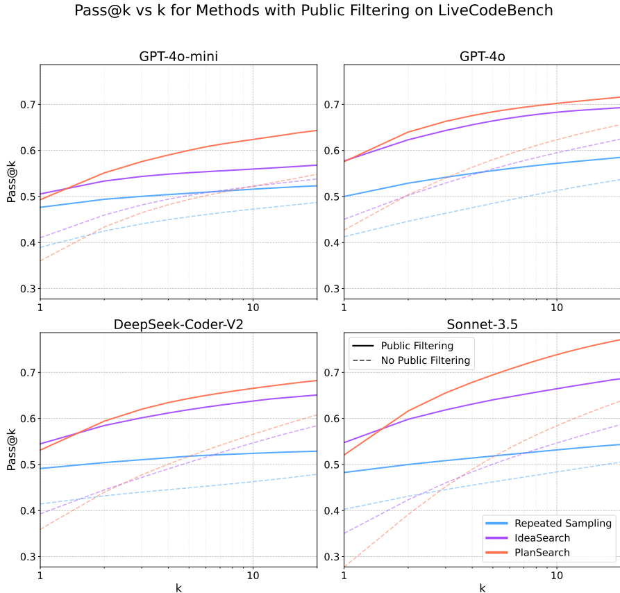
Figure 4: Performance of all models and methods on LiveCodeBench with public test filtering. The purpose of filtering is to shift pass@k curves leftward (i.e., bringing performance at high k to low k ), so we plot curves in detail over k \in \{1, \dots, 20\} . Even at 10 completions, PLANSEARCH outperforms filtered REPEATED SAMPLING by a flat 30 to 40%. Again, full pass@k plots are included in their entirety in Appendix A.
