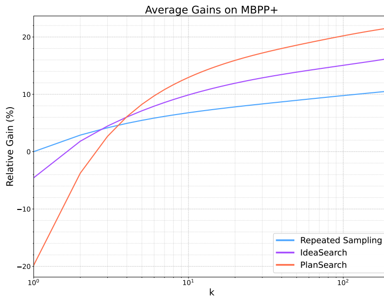
Figure 12: Performance gain over REPEATED SAMPLING@1 averaged over all models on MBPP+, plotted over k \in \{1, \dots, 200\} .
