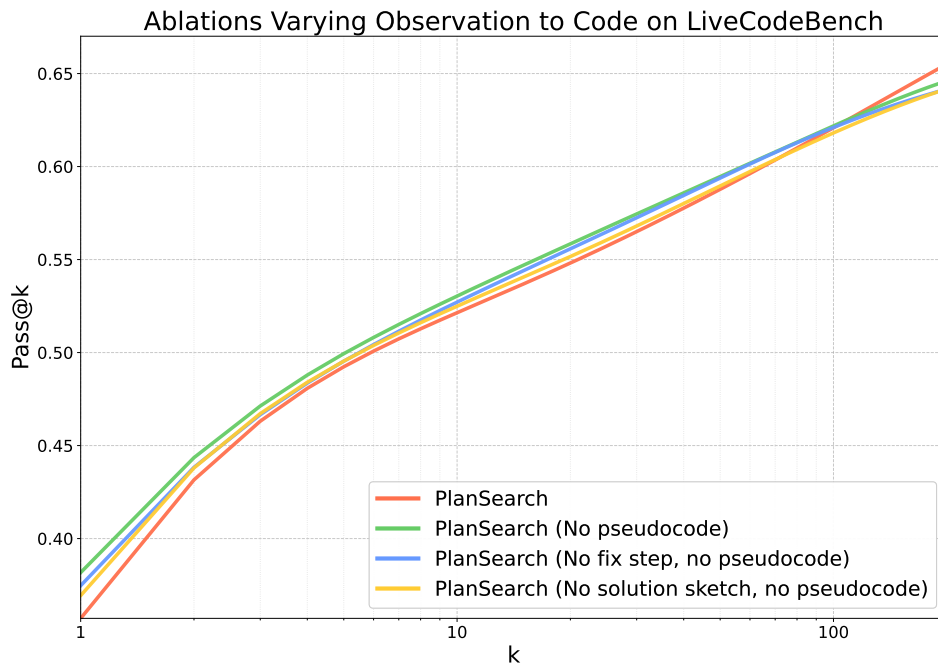
Figure 29: We run ablations of PLANSEARCH with different methods of translating a combination of observations to code.
