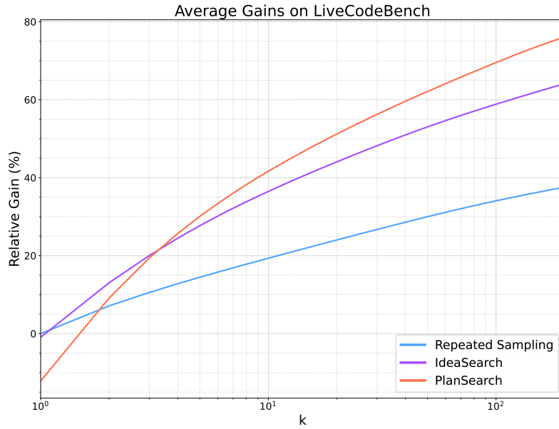
Figure 13: Performance gain over REPEATED SAMPLING@1 averaged over all models on LiveCodeBench, plotted over k \in \{1, \dots, 200\} .
