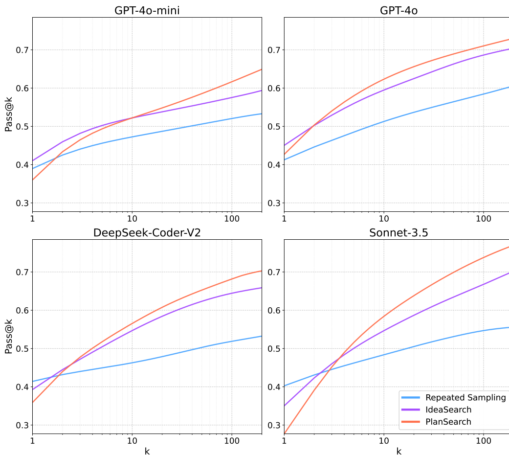
Figure 8: Pass@k performance of all models and methods on LiveCodeBench, plotted over k \in \{1, \dots, 200\} .
