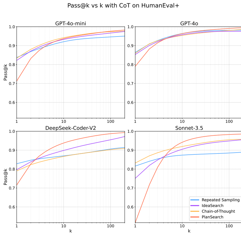
Figure 20: Pass@k graphs on HumanEval+, with the Chain-of-Thought baseline.
