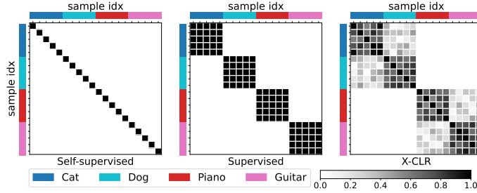
Figure 2: Sample similarity adjacency matrices of existing methods vs. our \mathbb{X} -Sample Contrastive similarity loss (right) . We show pairwise similarities of 20 samples belonging to 4 classes. Similarity of 1 means the samples are identical, 0 – they are completely unrelated. In case of self-supervised learning, none of the inter-sample relationships are modelled (left). Supervised learning relies on the labels to group samples of the same class together (center). \mathbb{X} -CLR models inter-class relationships by associating cats with dogs and pianos with guitars.
