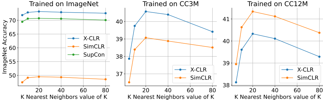
Figure 7: Results of models trained on ImageNet, CC3M, CC12M on ImageNet validation when using KNN classifier.
