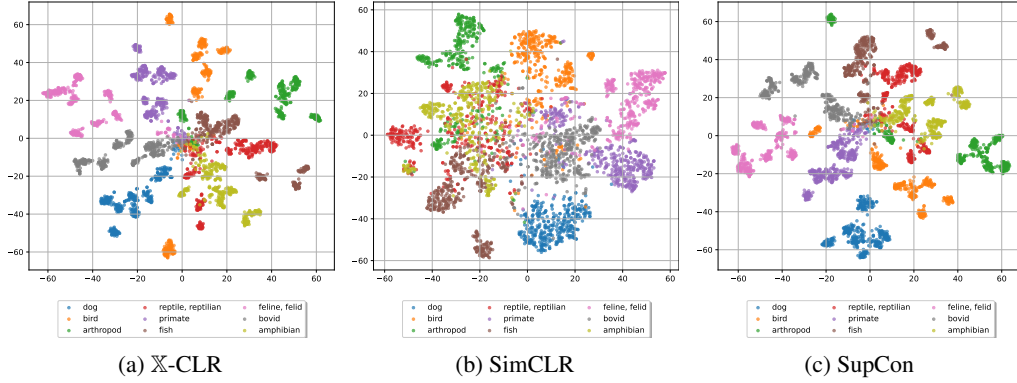
Figure 9: X-CLR and SupCon representations fall into well-defined clusters, whereas SimCLR representations are less structured.
