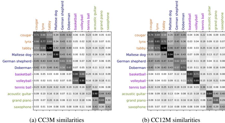
Figure 6: \mathbb{X} -CLR Learned similarities when trained on a) CC3M and b) CC12M.
