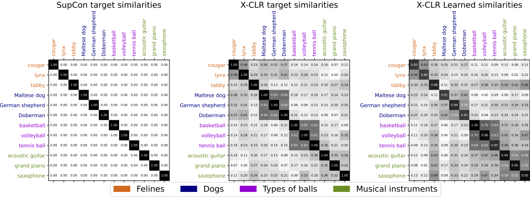
Figure 4: Visualizing pairwise similarities SupCon [Khosla et al., 2020] objective does not encourage non-zero similarity between samples of different classes (left), while X-CLR target similarities take into account semantic closeness within categories such as dogs or types of balls (center). On the right, we see that the trained model successfully learns the soft similarity. For more graphs, see fig. 5.
