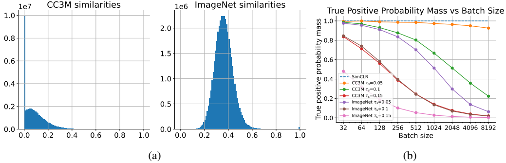
Figure 8: (a) Histograms of the similarities calculated using Sentence Transformer on ImageNet and CC3M. While for ImageNet the average similarity is around 0.35, it is much lower on CC3M, signifying that the graph contains less information for CC3M. (b) Effect of the temperature and batch size on the weight assigned to the true positive.
