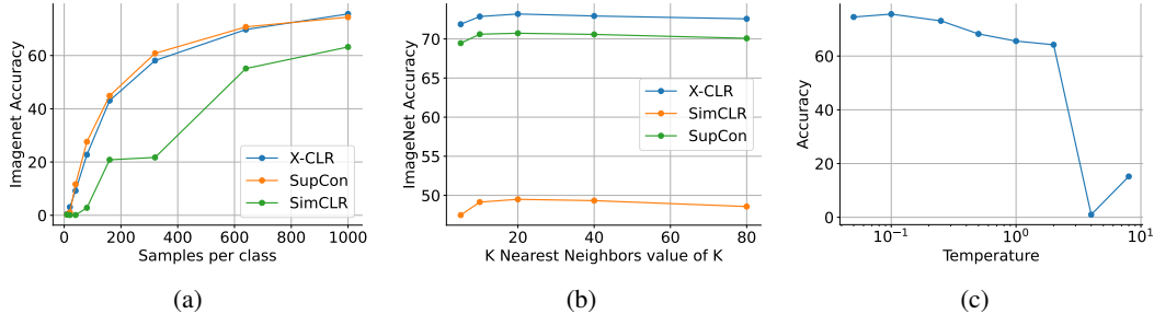
Figure 3: (a) \mathbb{X} -Sample Contrastive Loss is data efficient with ImageNet pretraining. We outperform SimCLR in low data regimes and match Supervised Contrastive trained on ground truth labels at varying levels of data scarcity. (b) KNN performance ImageNet. \mathbb{X} -CLR outperforms other methods with KNN probing for a range of values of K. (c) Sensitivity of \mathbb{X} -Sample Contrastive to temperature. We test the performance of our method when trained with different values of temperature \tau_s on ImageNet data.
