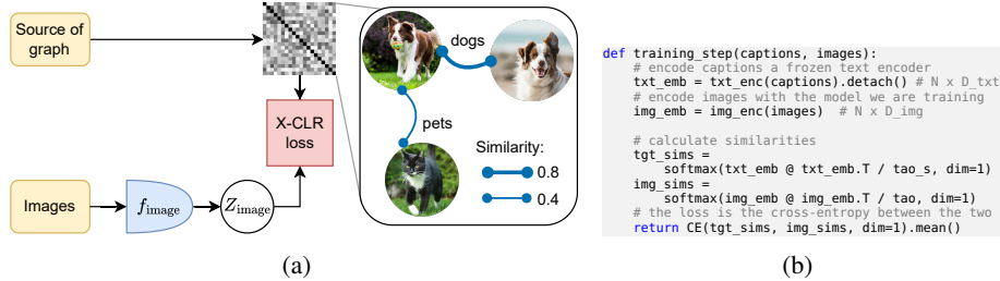
Figure 1: a) The diagram of \mathbb{X} -CLR. \mathbb{X} -CLR objective learns representations of images with the help of a soft relationship graph. The graph can be built based on accompanying data, e.g. taxonomy for biological data. In our experiments, we use captioned images, and build similarities based on the similarity of captions. b) Python-style pseudo-code of \mathbb{X} -CLR with similarity based on captions.
