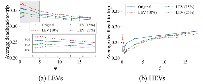
Figure 8: Average deadhead-to-trip distance ratio on y -axis for (a) LEVs and (b) HEVs, as a function of \phi on the x -axis for different LEV fractions. At higher \phi values, the deadhead-to-distance ratio for LEVs decreases but increases for HEVs.
