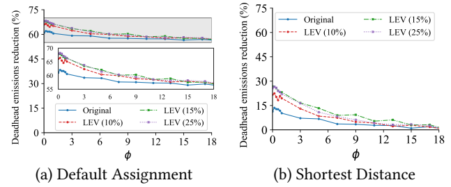
Figure 5: Percentage reduction in deadhead miles emissions on y-axis compared to the (a) default assignment in the RideAustin dataset and (b) shortest distance driver assignment, as a function of \phi on the x-axis for different LEV fractions. Lower values of \phi generally yield higher reduction.
