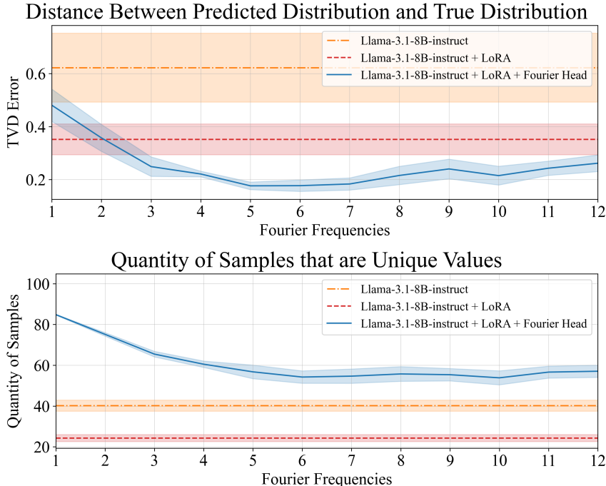
Figure 12: We demonstrate that the Fourier head model consistently obtains a lower total variation distance, as well as a greater diversity of samples. For TVD (top), lower is better, because lower values indicate that the learned distribution is closer to the ground truth distribution. And for quantity of samples (bottom), higher is better, because lower values indicate that the LM has just memorized specific numbers instead of performing sampling. We present here the mean values across the four distributions, for all ten seeds. We can see that the Fourier head obtains more diverse samples, and learns a distribution closer to the ground truth.
