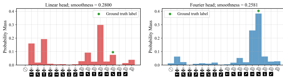
Decision Transformer Example: Learned Next Action Distributions
