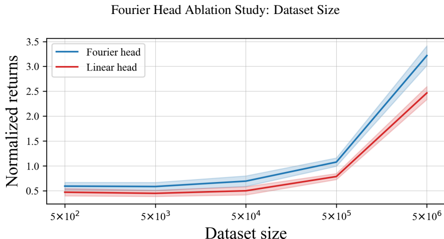
Figure 15: In this ablation study, we analyze whether dataset size has any effect on the relative performance of the Linear head and the Fourier head. Our results show that, across dataset sizes, the Decision Transformer agent with a Fourier head achieves larger returns than the linear head on the Seaquest game.
