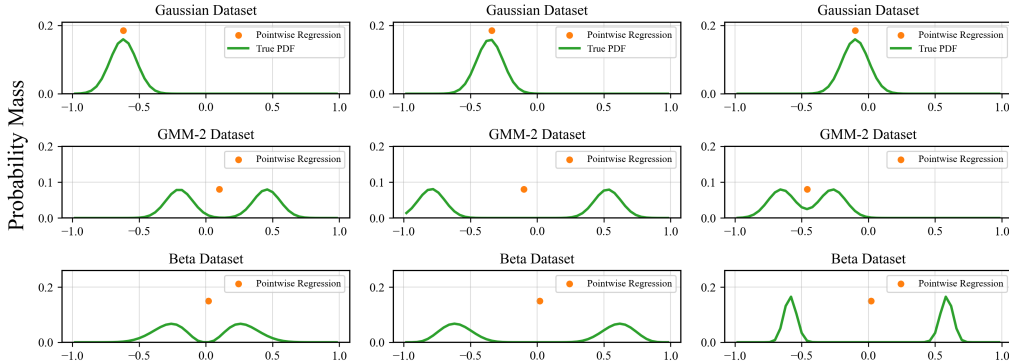
Toy Example: Ground Truth Conditional Distribution vs. Pointwise Regression Output
