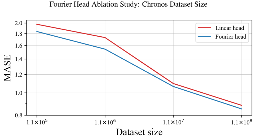
Figure 18: In this ablation study, we analyze whether dataset size has any effect on the relative performance of the linear head and the Fourier head for the probabilistic time series task. Our results show that, across dataset sizes, the Fourier head yields more accurate forecasts than the linear head . For the dataset sizes 1.1 \times 10^5 , 1.1 \times 10^6 , and 1.1 \times 10^7 , we report the average MASE across four seeds; for the dataset size 1.1 \times 10^8 we report the MASE from Table 3. We generate the plot following (Kaplan et al., 2020) and observe a similar power-law scaling behavior for both methods, with the Fourier head consistently outperforming the linear head.
