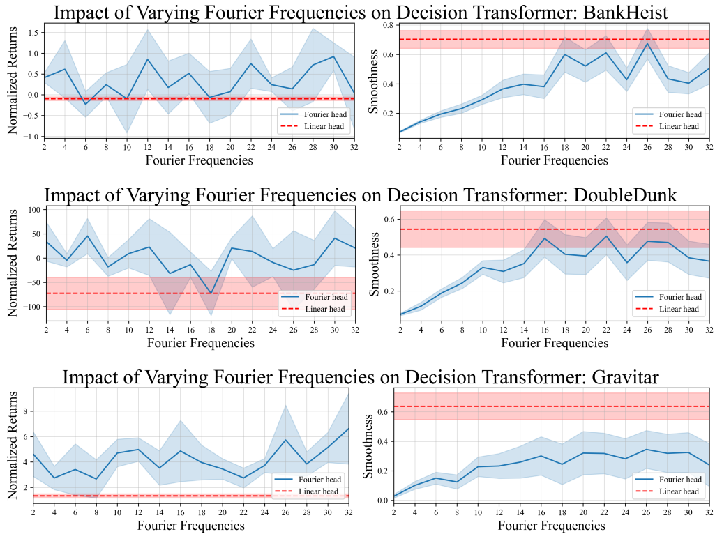
Figure 16: We present empirical results for how the quantity of Fourier frequencies impacts returns and smoothness for additional imitation learning games. For normalized returns, higher is better; for smoothness, lower is better. We can see that for the BankHeist, DoubleDunk, and Gravitar games, the Fourier agent consistently achieves higher normalized returns than the linear baseline agent, while still learning smoother next-action distributions.
