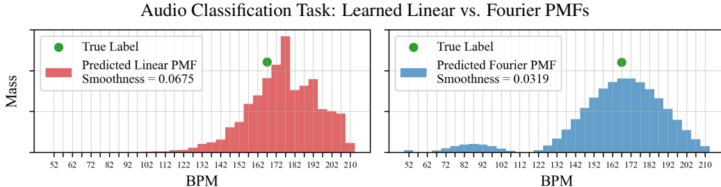
Figure 7: Comparison between the PMF learned by the linear head , and the Fourier head with 2 frequencies, for the toy BPM classification task, on a single audio example . We observe that the Fourier head learns a smoother categorical distribution over its predicted values, and is better centered around the ground truth label . We also note the small mini-sine wave artifacting on the left side of the Fourier model, which tends to occur when using few frequencies.
