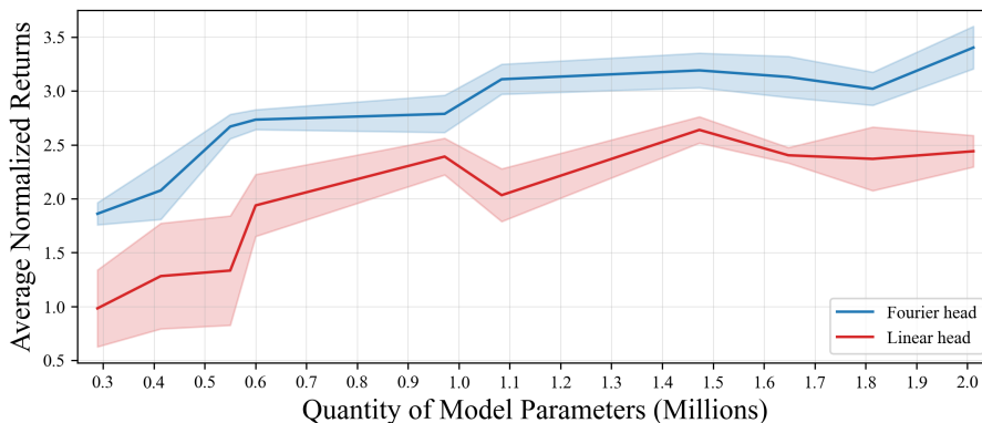
Impact of Model Size on Decision Transformer Returns: Seaquest
