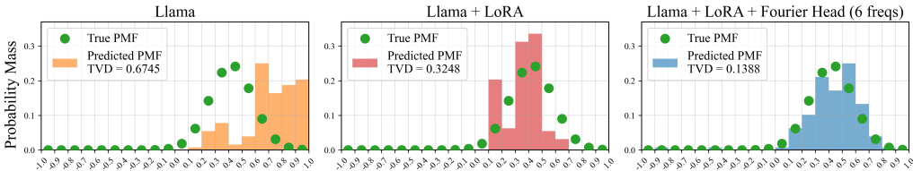
Using Llama-3.1-8B-Instruct to Simulate Gaussian Sampling
