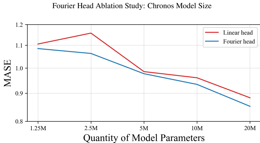
Figure 19: In this ablation study, we analyze whether model size has any effect on the relative performance of the linear head and the Fourier head for the probabilistic time series forecasting task. Our results show that, across model sizes, the Fourier head yields more accurate forecasts than the linear head . For the model sizes 1.25M, 2.5M, 5M, and 10M, we report the average MASE across three seeds; for the model size 20M we report the MASE from Table 3. We generate the plot following (Kaplan et al., 2020) and observe a similar power-law scaling behavior for both methods, with the Fourier head consistently outperforming the linear head.
