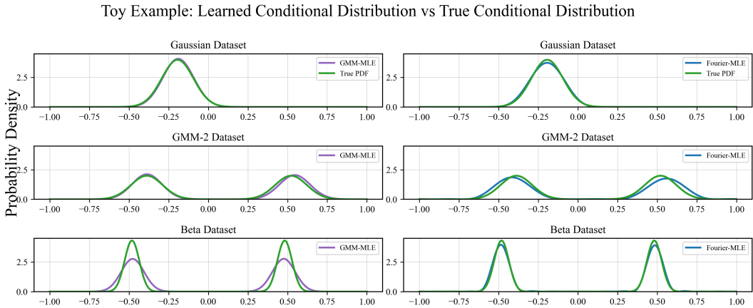
Figure 11: Comparison between the PDFs learned by the GMM-MLE head and the Fourier-MLE head for each of the datasets in the toy example. While GMM-MLE outperforms Fourier-MLE on the Gaussian and GMM-2 datasets, Fourier-MLE performs better on the Beta dataset.
