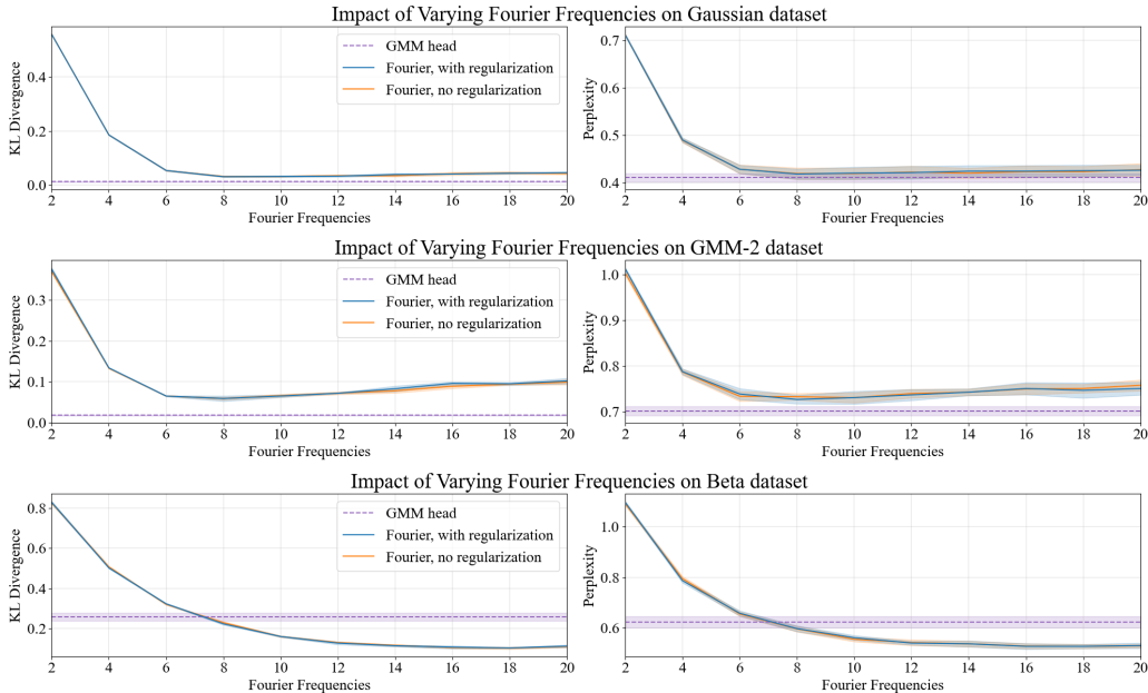
Figure 9: We study how the quantity of Fourier frequencies impacts KL divergence and perplexity for the toy example on each dataset for the MLE experiments. For both KL divergence and perplexity, lower is better. We observe that the Fourier models with and without regularization performed similarly to each other. While the GMM head has better KL divergence on the Gaussian and GMM-2 datasets, which is to be expected, the Fourier model (both with and without regularization ) has the best KL divergence on the Beta dataset for sufficiently large Fourier frequencies, since it is non-Gaussian.
