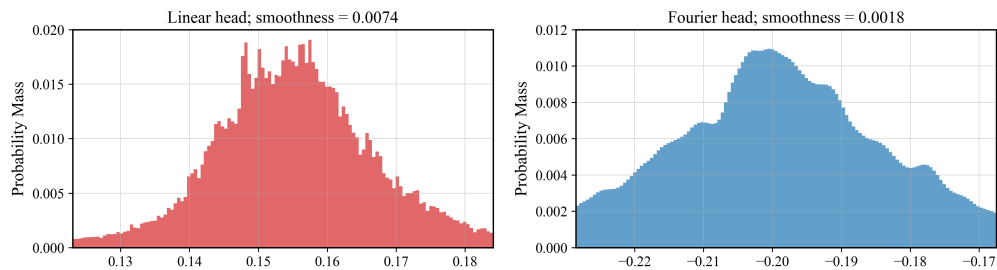
Chronos Example: Learned Token Distribution
