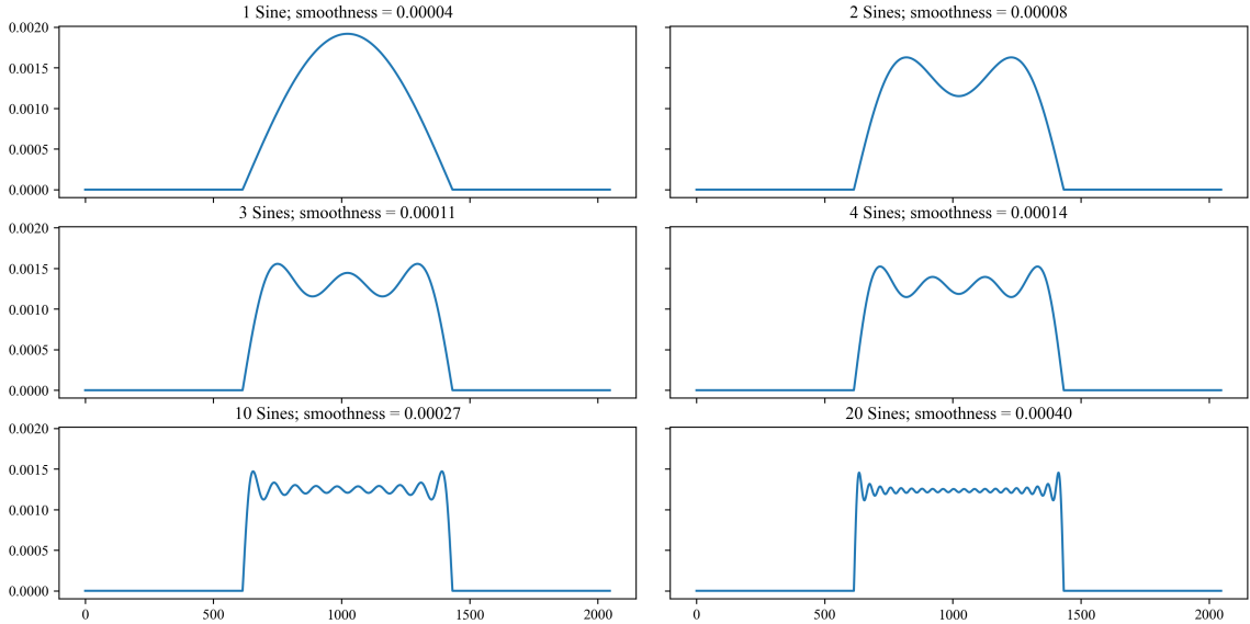
Figure 5: Truncated square waves framed as densities and their smoothness.
