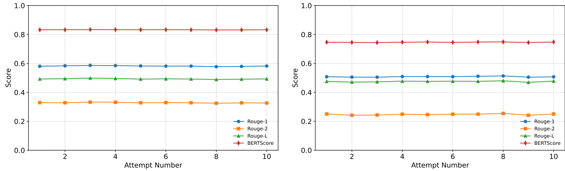
Figure 2: Performance of our model over ten resampling trials on the test datasets of CSDS and SAMSum
