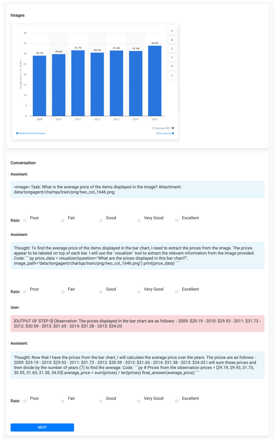
Figure 5: The interface of the user study for data quality.
