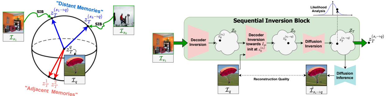
Figure 7. The many memories of an ablated image: (Left) The latent seed z_T^q of the query image \mathcal{I}_q can be obtained from various support images: \mathcal{I}_{s_1}, \dots, \mathcal{I}_{s_k} . For support image \mathcal{I}_{s_i} , we apply the sequential inversion block shown on the right to map it to the seed z_T^{(s_i \rightarrow q)} . We show in Fig. 5 that seeds \{z_T^{(s_i \rightarrow q)}\}_{i=1}^k are likely enough and can be used to generate the query image \mathcal{I}_q . (Right) Recovering the seed of a query image \mathcal{I}_q when starting with support image \mathcal{I}_{s_i} .
