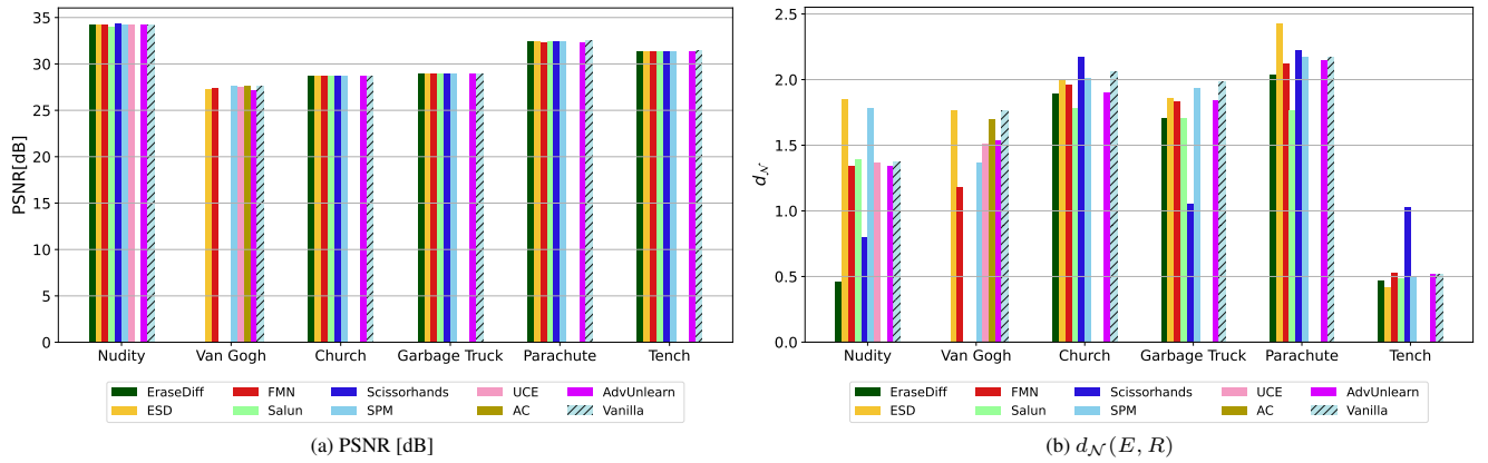
Figure 5. A concept erased model remembers: We report the mean reconstruction PSNR (a) and our proposed relative distance (b) for six concept datasets {Nudity, Van Gogh, Church, Garbage Truck, Parachute, Tench} across nine different concept ablation methods {EraseDiff [45], ESD [7], FMN [47], Salun [4], Scissorhands [44], SPM [23], UCE [8], AC [19], AdvUnlearn [49]}, along with one “Vanilla” SD 1.4 [31] model. These results validate that, at the dataset level, there exists at least one latent per image that can reconstruct the image with high quality ( \text{PSNR} \geq 25 dB) from a reasonable likelihood using the concept erased model.
