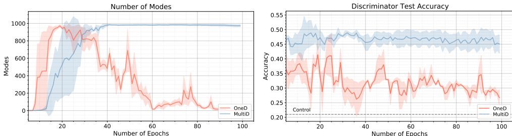
Figure 2: Investigating the forgetting-collapse interplay: We investigate our hypothesis that catastrophic forgetting is associated with mode collapse. To this end, on the left pane, we plot the magnitude of mode collapse by counting the number of modes produced by the generator. On the right pane, we assess the quality of the discriminator features by plotting the accuracy of linear classifier on top of the discriminator features at each epoch. In the original DCGAN model ( OneD ), the coverage of modes and the quality of discriminator features are both low and decreasing. In particular, the test accuracy from the discriminator’s features drops almost to randomly initialized weights (shown as control ). On the other hand, adding DMAT ( MultiD ) dramatically improves both mode coverage and the discriminator test accuracy.
