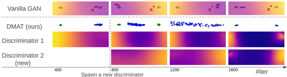
Figure 1: Visualizing training trajectories: We visualize the distribution of the real (green dots) and fake (blue dots) over the course of the vanilla GAN (top row) and our method (the second row and below). The background color indicates the prediction heatmap of the discriminator with blue being fake and warm yellow being real. Once the vanilla GAN falls into mode collapse (top row), it ends up oscillating between the two modes without convergence. Moreover, the discriminator’s prediction at point X oscillates, indicating catastrophic forgetting in the discriminator. With our DMAT procedure, a new discriminator is dynamically spawned during training. The additional discriminator effectively learns the forgotten mode, guiding the GAN optimization toward convergence.
