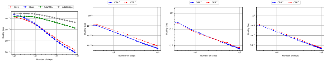
(a) Matrix game. (b) EFG: Leduc, 2 players, 9 ranks. (c) EFG: Battleship, 3 turns, 1 ship. (d) EFG: Leduc, 2 players, 5 ranks.
