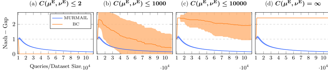
Figure 2: Empirical evaluation for environments with different C(\mu^E, \nu^E) .
