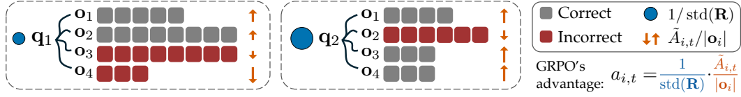
Figure 4: Illustration of the biases in GRPO. Note that the effective advantage of GRPO a_{i,t} is equivalent to a reweighted version of the unbiased advantage \hat{A}_{i,t} = R(\mathbf{q}, \mathbf{o}_i) - \text{mean}(\mathbf{R}) . The terms \text{std}(\mathbf{R}) and |\mathbf{o}_i| could bias the optimization by assigning different weights to different questions and responses, as denoted by the sizes of the blue circles and the lengths of the orange arrows. Upward arrows indicate positive advantages, and vice versa.
