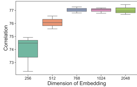
Figure 10: Impact of dimensions of the sentence embedding.
