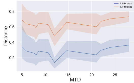
Figure 4: L1 and L2 distances of learned embedding’s uniformity and alignment with a fixed point changes along with MTD.
