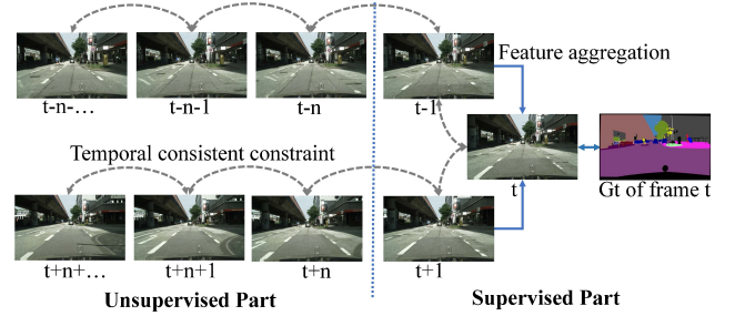
Figure 1: Illustration of a video snippet that contains 30 frames with only one annotated frame t . Unlike previous models that only utilize those frames close to the frame with ground-truth by feature aggregation (solid lines), our model makes full use of all frames in the video with temporal consistent constraints (dashed lines).
