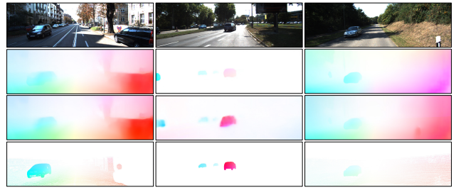
Figure 5: Visual comparison on the KITTI dataset for optical flow. From top to bottom: original images, our results, GeoNet (Yin and Shi 2018) and ground truth. Our model estimate sharper motion boundaries than GeoNet. The middle column is an occluded case that the car is driving out of the camera scope, our model accurately handles the occlusion.
