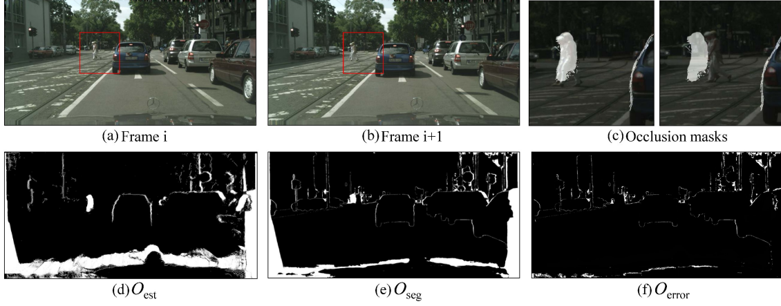
Figure 3: Two types of occlusion masks are applied in our model. (c) shows the zoom-in occlusion masks inside the red rectangle region of (a). (d) is the occlusion mask O_{\text{est}} which is estimated by the non-occluded flow branch. (e) is the occlusion mask O_{\text{seg}} obtained from the inconsistency of the segmentation maps. The error mask O_{\text{error}} is shown in (f).
