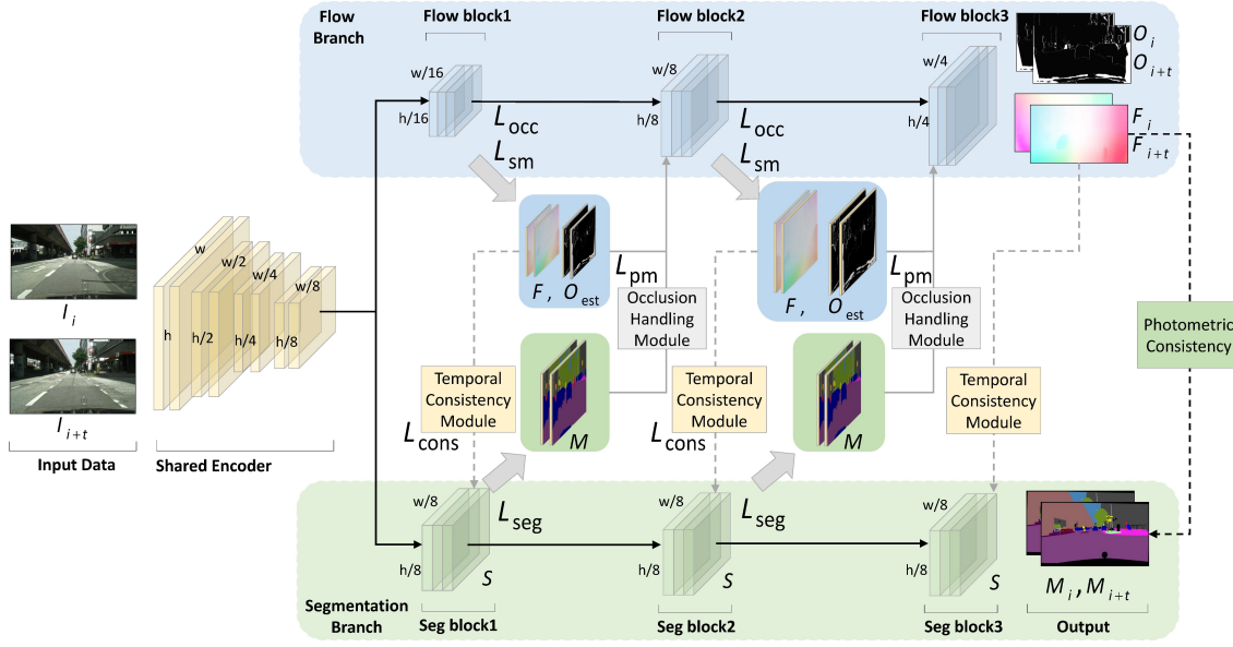
Figure 2: The overall pipeline of our joint learning framework. The blocks represent the feature maps of our model, the gray dashed line represents the temporally consistent constraints. The gray solid line represents the occlusion handling module with the inconsistency of the segmentation maps.
