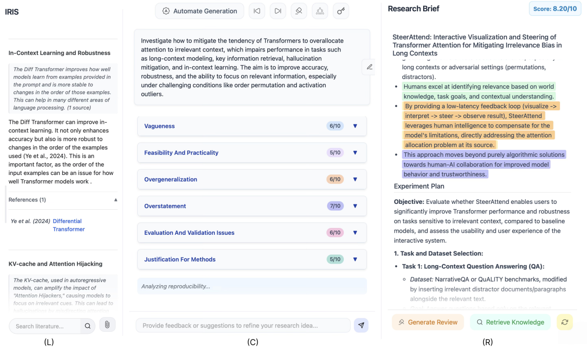
Figure 2: IRIS Platform Interface with (L) Retrieval Panel, (C) Chat Overview Panel, (R) Research Brief Panel
