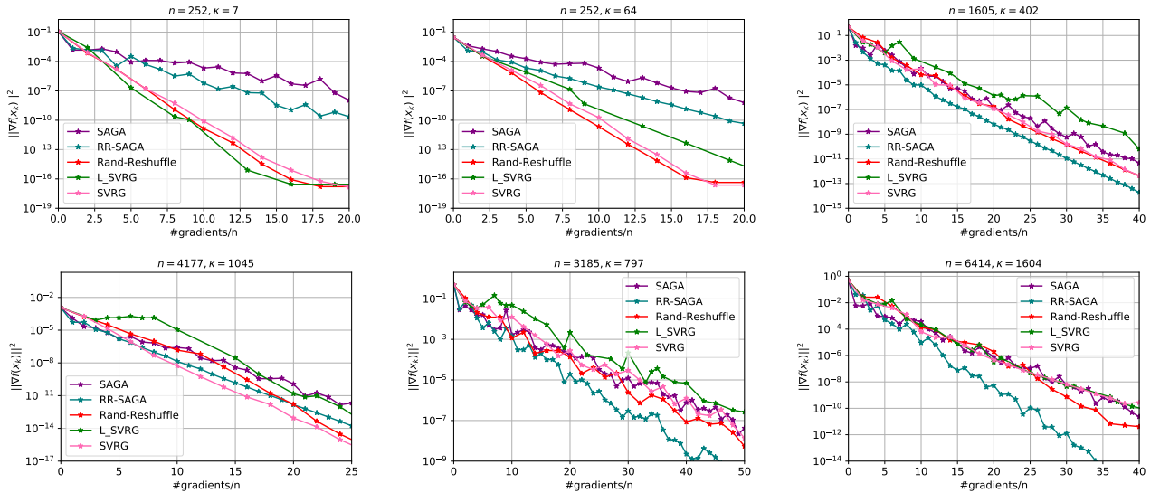
Figure 4: Comparison of SAGA, RR-SAGA, Rand-Reshuffle, L-SVRG and SVRG with optimal stepsizes on bodyfat dataset with different regularization constants (upper left and middle), a1a (upper right), aba1one (lower left), a3a (lower middle) and a5a (lower right).
