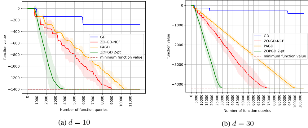
Figure 1: Performance on toy octopus function, with \tau = e, L = e, \gamma = 1 (Here, \tau, L, \gamma are parameters determining the properties of f . Our parameter choice is consistent with that in Zhang et al. (2022). See Du et al. (2017) for details about the definitions of \tau, L and \gamma .)
