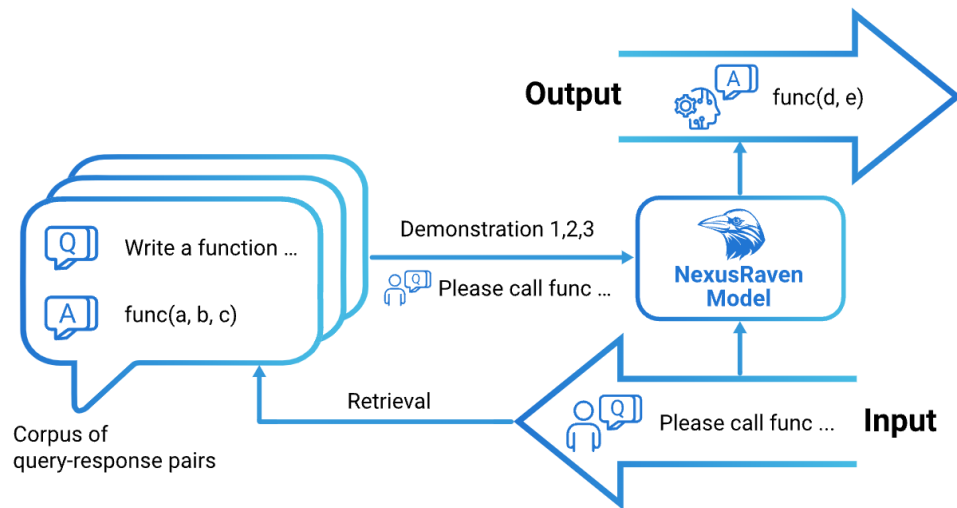
Figure 3: Illustration of our demonstration retrieval augmentation system. When presented with a new query, our system scans an existing corpus to identify demonstration examples that can enhance the quality of responses to that query.
