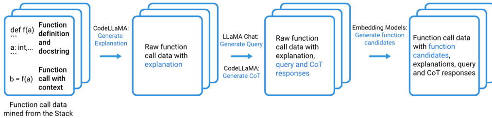
Figure 2: Illustration of our multi-step refinement pipeline.
