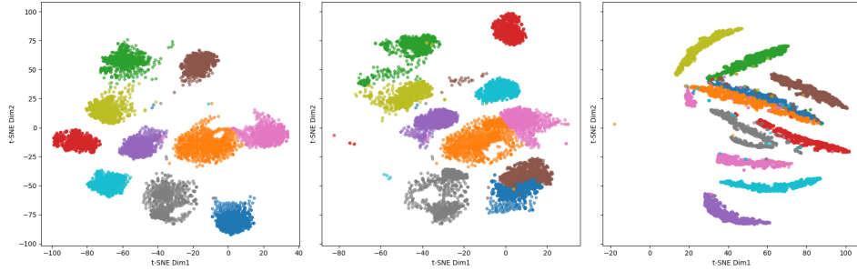
(b) NegGrad: t-SNE visualizations before and after objective-level unlearning on DINOv2 features. Left: original embedding space. Middle: after injecting arbitrary objective. Right: after NegGrad-based unlearning. Class structure is not recovered.
