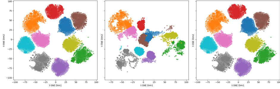
(a) COU: t-SNE visualizations before and after objective-level unlearning on DINOv2 features. Left: original embedding space. Middle: after injecting arbitrary objective. Right: after COU unlearning. COU restores clean cluster structure.
