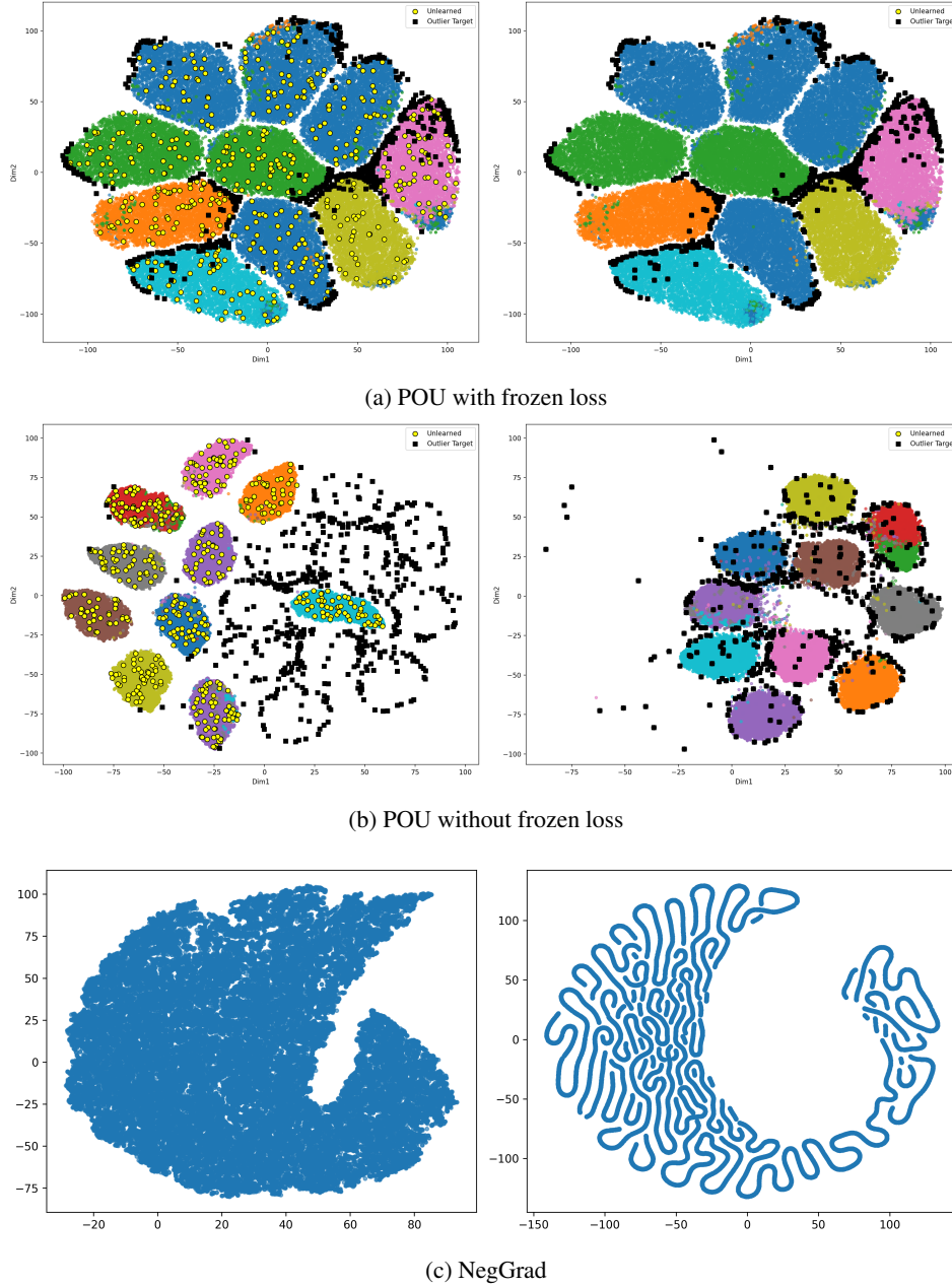
Figure 3: t-SNE visualizations of instance-level unlearning on CIFAR10. The comparison illustrates the importance of the frozen loss in POU. With frozen loss (top), cluster structures are preserved and unlearned samples are cleanly displaced to outlier regions. Without frozen loss (middle), forgetting is incomplete and retained clusters are distorted. NegGrad (bottom) shows severe representation collapse and poor separation.
