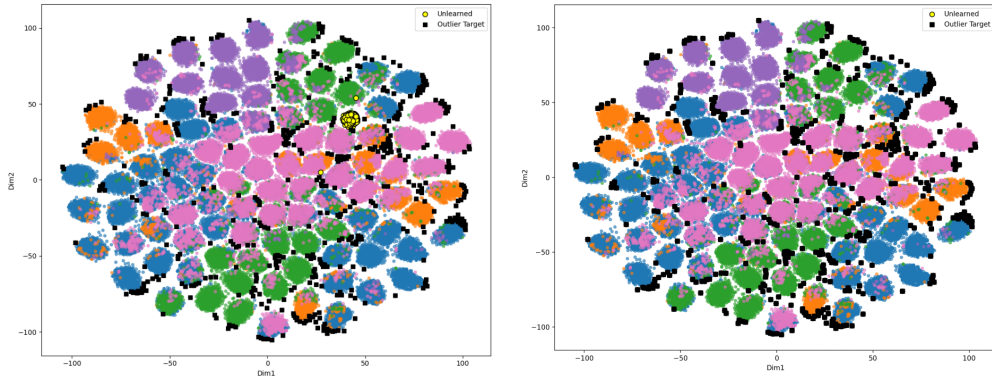
Figure 5: t-SNE visualization of class-level unlearning on CIFAR100 using POU. Left: The original projection space before unlearning shows well-separated latent subclusters for each class. Right: After unlearning, the deleted class samples (yellow) are successfully displaced to synthetic outlier regions (black squares), while the rest of the latent structure remains stable. This confirms that POU achieves class forgetting without disturbing non-target data.
