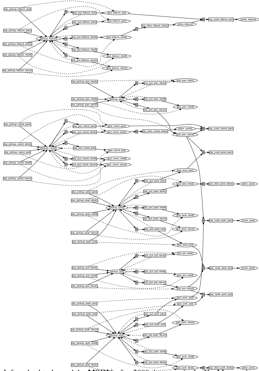
Figure 8: Inferred subtask graph by \text{MSGI}^+ after 2000 timesteps in the Cooking environment. For \text{MSGI}^+ , 262 options with no inferred precondition and effect were not visualized for readability. Options are represented in rectangular nodes. Subtask completions and attributes are in oval nodes. A solid line represents a positive precondition / effect, dashed for negative. Ground truth attributes are included option/subtask parameters, however which attributes are used for which option preconditions is still hidden, which \text{MSGI}^+ must infer.
