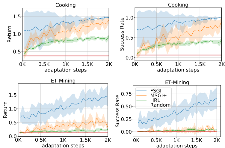
Figure 4: The adaptation curves in the Cooking and Mining domains.
