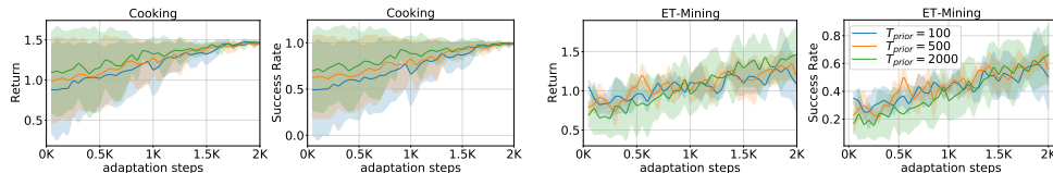
Figure 7: The adaptation curve of PSGI trained with different priors. Priors were trained in the training tasks of Cooking and Mining domains respectively for T_{prior} = 100, 500, \text{ and } 2000 timesteps.
