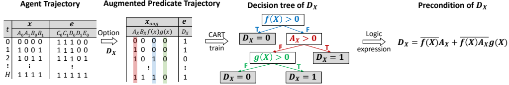
Figure 2: An overview of our approach for estimating the parameterized precondition of the subtask graph \widehat{\mathcal{G}}_{\text{prec}} in a simple environment with subtasks A, B and options C, D, E . Each subtask and option has a parameter 0 or 1. Note by inferring the parameterized precondition and effects, we can infer the behavior unseen subtasks and options such as D_2 . We run precondition inference for every option and show D_X as an example. 1. The first table is built from the agent’s trajectory ( x is the subtask completion, e the option eligibility). 2. We build the second table, the “augmented” trajectory by substituting X into all possible subtask completions, A_X, B_X , and inferred attributes f, g . 3. We train a decision tree over the table, to infer the relation x_{\text{aug}} \rightarrow D_x (predicting when D_x is eligible given the completion x_{\text{aug}} ). 4. We translate the decision tree into an equivalent predicate boolean expression, which is one part of the inferred parameterized subtask graph \widehat{\mathcal{G}} .
