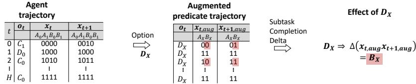
Figure 5: An overview of our approach for estimating the parameterized effect of the parameterized subtask graph, \widehat{\mathcal{G}}_{\text{eff}} , in a simple environment with subtasks A, B and options C, D, E . Each subtask and option has a parameter 0 or 1. We run effect inference for every option and show D_X as an example. 1. The first table is built from the agent’s trajectory ( x_t, o_t is the subtask completion and option executed at time t ). 2. We build the second table, the “augmented” trajectory by substituting X into all possible subtask completions, A_X, B_X , and restricting the table to only row where o_t = D_X . 3. We infer option dynamics, (x_t, o_t) \mapsto x_{t+1} , by calculating the simple aggregated difference between subtask completion before and after D_X , \Delta(x_{t,aug}, x_{t+1,aug}) .
