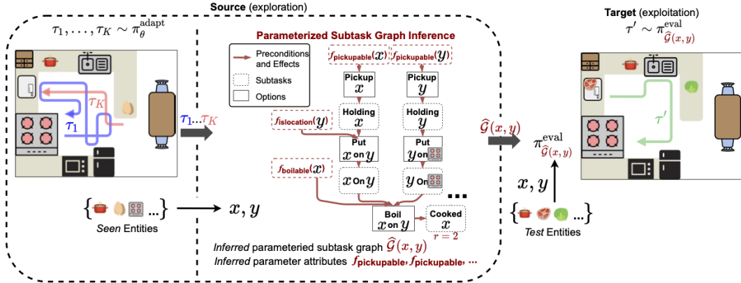
Figure 1: Illustration of parameterized subtask graph inference (PSGI) in a toy cooking environment. In various tasks, the agent must cook various foods to receive reward. Left: The adaptation policy \pi_{\theta}^{\text{adapt}} initially explores the cooking source task (training), generating a trajectories \tau_1, \dots, \tau_K . Mid- dle: Using \tau_1, \dots, \tau_K , the agent infers a parameterized subtask graph \hat{G}(x, y) of the environment, which describes the preconditions and effects between parameterized options and subtasks for any x and y , entities in the environment. The agent learns a set of parameter attributes ( \hat{A}_{\text{att}} = f_{\text{pickupable}} \dots ) in a zero-shot manner and uses these attributes to construct \hat{G} . Right: The agent initializes a separate test policy \pi_{\hat{G}}^{\text{test}} that maximizes reward by following the inferred parameterized subtask graph \hat{G} . In this target environment (test) there exist unseen parameters (cabbage and meat). Preconditions and effects for these parameters are accurately inferred by substituting for entities ( x and y ).
