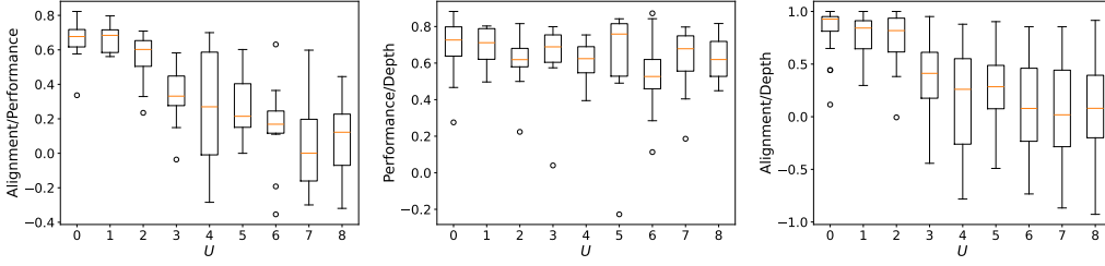
Figure 6: Alignment, performance, and depth correlation plots across different synthetic depths and experiment seeds. In each plot, we show the spread of Spearman correlation coefficients \rho for each level of uniqueness, where the orange lines are the median correlations and the dots are outliers. Left: When the two modalities are fully redundant, the alignment is strongly correlated with performance. When the two modalities have high uniqueness, alignment has a vanishing correlation with performance. In fact, for a significant proportion of tasks, the correlation is negative. Mid: In contrast, model size measured by depth always has a strong positive correlation with performance and does not seem to change across datasets. This means that representation alignment may not be a universal phenomenon, and is introduced by some special properties of data. In contrast, the influence of model size on performance seems universal and is consistent with the well-observed scaling laws. Right: For each level of uniqueness, we show the variance in alignment/depth correlation. As uniqueness increases, the median alignment/depth decreases to 0, and the range of correlation values increases significantly.
