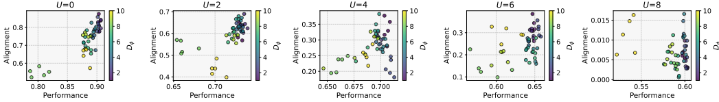
Figure 8: Alignment vs performance across levels of heterogeneity. We plot the alignment and performance scores at different levels of heterogeneity, with the transformed modality’s encoder fixed to the maximum transformation depth. At high levels of uniqueness, we see that high performance correlates with high alignment, with both being greater at lower synthetic depths. Past U = 4 , we see that while performance is higher at lower synthetic depths, the alignment scores on these datasets are not necessarily higher.
