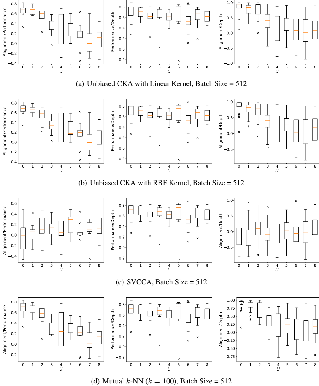
Figure 17: Alignment, performance, and depth correlation plots across different synthetic depths and experiment seeds with batch size = 512. In each plot, we show the spread of Spearman correlation coefficients \rho for each level of uniqueness.
