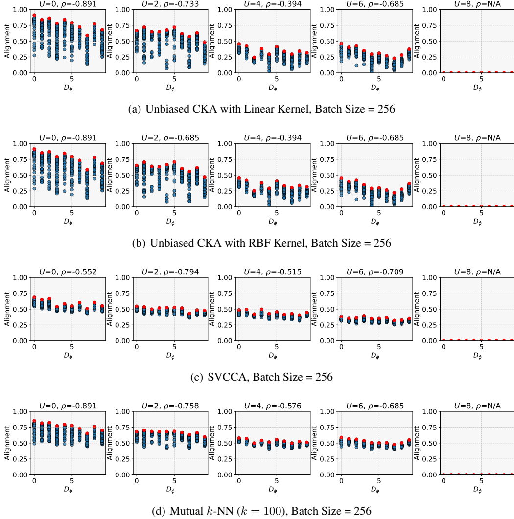
Figure 13: Alignment vs heterogeneity for various representation similarity metrics with batch size = 256. Spearman correlation coefficient \rho is computed between the maximum alignment, shown in red, and heterogeneity. N/A denotes that \rho is undefined as all alignment values are 0.
