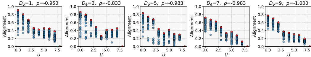
Figure 3: Alignment vs uniqueness on synthetic datasets. Alignment is computed between unimodal encoders trained on datasets with different levels of informational uniqueness U . Each dot is an independent run on a different model size on a given dataset. We see that the maximum level of achievable alignment, shown by the red dots, decreases as the level of uniqueness increases. Five different figures shows the different levels of nonlinear transformation we apply to the original data. We report the Spearman correlation \rho between the maximum alignment values and U .
