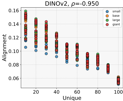
Figure 4: Alignment vs uniqueness on real large-scale vision-language datasets. Alignment is computed between DINOv2 vision models and large language models. Each dot is an independent run on a different model size on a dataset with a given level of uniqueness. The maximum achievable alignment decreases as uniqueness increases.
