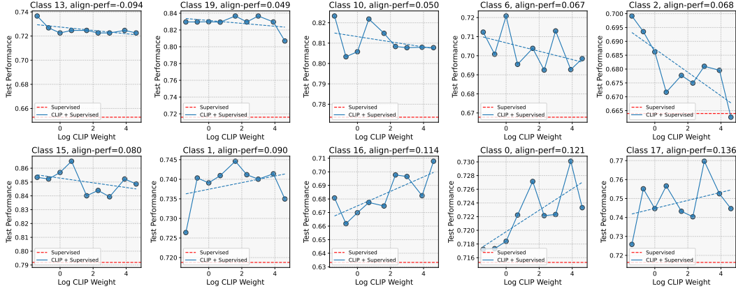
Figure 28: Alignment-performance relation predicts impact of explicit alignment on downstream performance on MM-IMDb. We consider a scenario where we only have a small subset (1k examples) of labeled training data and a full training dataset (15k examples) of paired images and text. One approach is to finetune a pretrained vision-language model with a loss combining a supervised objective, \mathcal{L}_{sup} , and an explicit alignment objective to achieve better generalization. In practice, we use the CLIP loss, \mathcal{L}_{CLIP} , for explicit alignment. Starting with vision and language models pretrained with CLIP, we finetune the vision and language encoder on MM-IMDb using \mathcal{L} = \mathcal{L}_{sup} + w * \mathcal{L}_{CLIP} , where \mathcal{L}_{sup} is computed with a linear layer on top of the language embeddings and the contribution of \mathcal{L}_{CLIP} is modulated by a weight w , where w \in \{0, 0.1, 0.25, 0.5, 1.0, 2.0, 5.0, 10.0, 50.0, 100.0\} . Left-to-right, top-to-bottom: The classification tasks are ordered by increasing alignment-performance linear fit slopes, which are computed on the sampled data using unimodal language and vision models. The dotted blue line shows the linear fit to performance across varying degrees of explicit alignment, and the dotted red line shows that finetuning with only \mathcal{L}_{sup} results in overfitting. Results demonstrate that alignment-performance relations predict how the amount of explicit alignment (controlled by w ) impacts performance. Specifically, classes 13, 19, 10, 6, 2, 15 have smaller alignment-performance linear fit slopes, which correspond to a weak or negative relation between w and performance. In contrast, classes 1, 16, 0, 17 have higher alignment-performance linear fit slopes, in which case increasing w generally improves performance.
