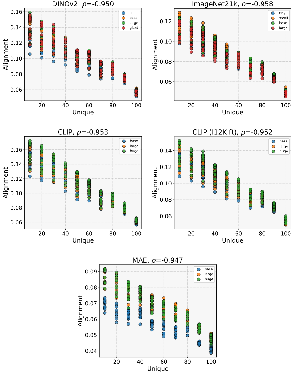
Figure 26: Vision-Language Alignment vs Uniqueness. The alignment is computed between various vision models and large language models. We compute the Spearman correlation coefficient \rho between the maximum alignment and uniqueness.
