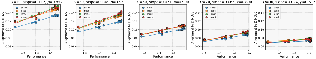
Figure 7: Alignment vs performance across different uniqueness. We plot the vision-language alignment using DINOv2 vision models with respect to language model performance, measured using negative bits-per-byte-loss. We show individual best fit lines for each size of vision model and the average Spearman correlation coefficient \rho . As U increases, the slope of the linear fit decreases, showing that better performance can be achieved without increased alignment.
