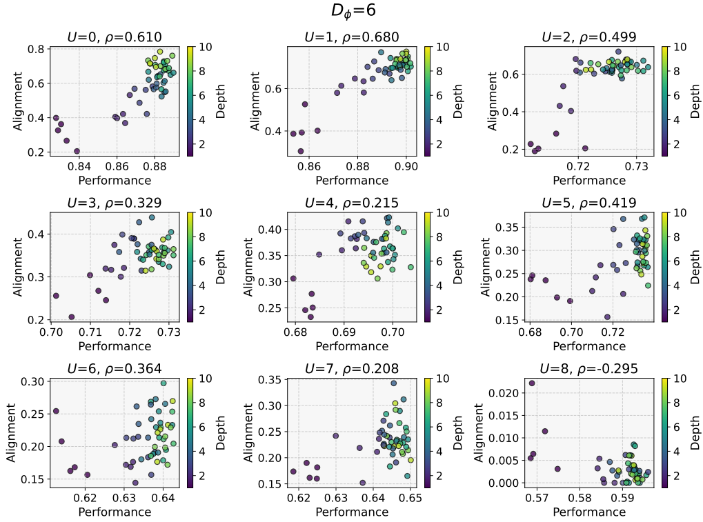
Figure 24: Alignment vs Performance for D_\phi = 6 . The alignment-performance trend is shown across different levels of uniqueness, with the Pearson’s correlation coefficient r reported for each plot.
