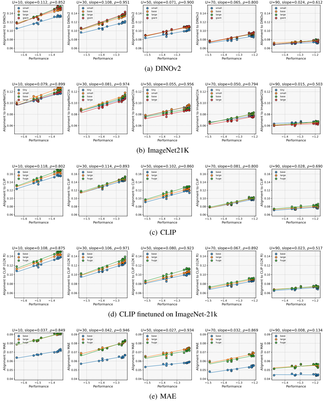
Figure 27: Vision-Language Alignment vs Performance. We plot the vision-language alignment using various vision models with respect to language model performance, measured using bits-per-byte-loss and show individual best fit lines for each size of vision model as well as the average Spearman correlation coefficient \rho . As U increases, the relation between alignment and performance weakens.
