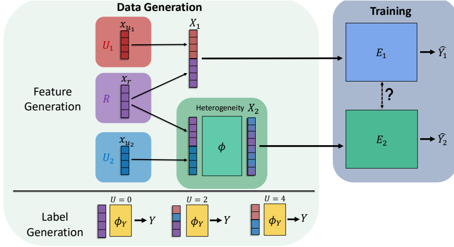
Figure 2: Synthetic data generation and training. We generate synthetic data with varying levels of uniqueness and heterogeneity. The building blocks are the redundant and unique components [x_r, x_{u1}, x_{u2}] , where [x_r, x_{u1}] are used in creating X_1 and [x_r, x_{u2}] are for X_2 . The level of uniqueness is determined by the number of features from x_r that are used to compute the labels Y , given that the total number of features used for label computation is held constant. X_2 is transformed into a heterogeneous modality using a transformation network \phi . In our experiments, we compute alignment between unimodal encoders E_1, E_2 trained on X_1, X_2 respectively.
