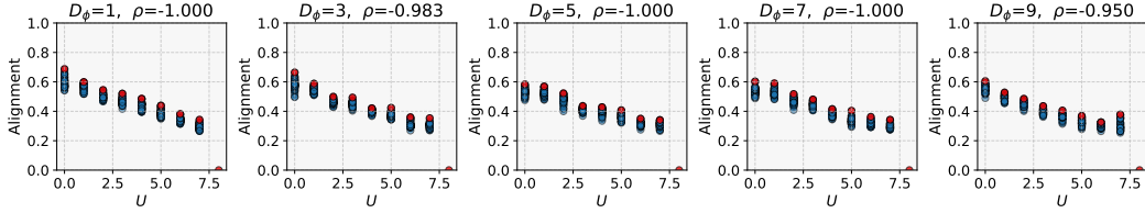
(c) SVCCA, Batch Size = 256
