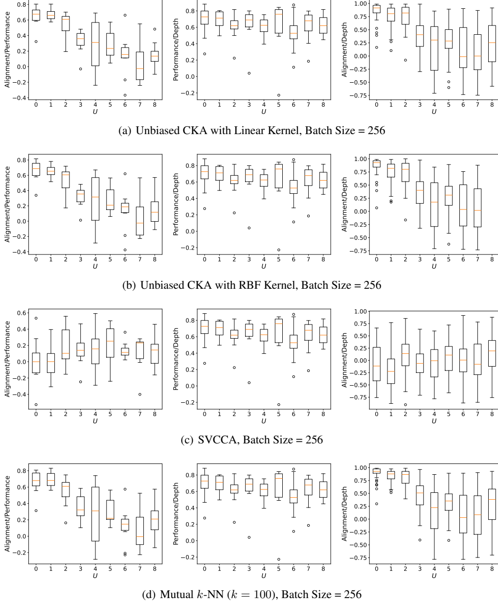
Figure 16: Alignment, performance, and depth correlation plots across different synthetic depths and experiment seeds for various representation similarity metrics with batch size = 256. In each plot, we show the spread of Spearman correlation coefficients \rho for each level of uniqueness.
