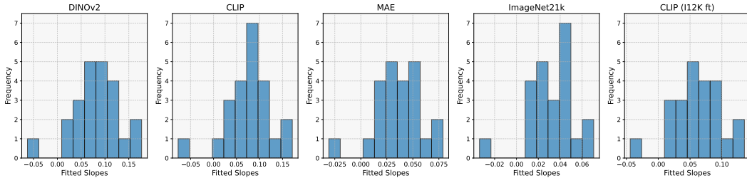
Figure 9: Relationship between alignment and performances across MM-IMDb classification tasks. Using the same set of language and vision models as Huh et al. (2024), we evaluate cross-modal alignment on MM-IMDb (Arevalo et al., 2017), a dataset for movie genre prediction, where we consider two modalities: images of the movie poster and text of the plot descriptions. The task is multi-label classification with 23 categories, as movies can be labeled as one or more genres. To measure performance for each language model, we train a linear classification layer on the last layer hidden representations. We plot the slope of the linear fit to the alignment-performance scores across categories, which varies due to different levels of information content required for each downstream classification task.
