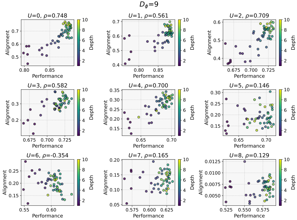
Figure 25: Alignment vs Performance for D_\phi = 9 . The alignment-performance trend is shown across different levels of uniqueness, with the Pearson’s correlation coefficient r reported for each plot.
