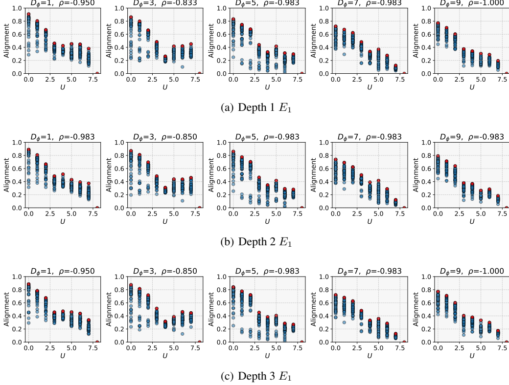
Figure 19: Alignment vs uniqueness for various depths of E_1 . The distribution of alignment scores for various depths of E_1 are nearly identical, as a single level neural network is sufficient to model the untransformed modality.
