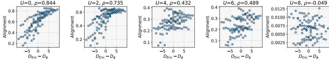
Figure 5: Emergence of alignment across heterogeneity and uniqueness. We plot alignment with respect to (D_{Enc} - D_\phi) for different levels of uniqueness and report the Spearman correlation \rho . When redundancy is high, we see that alignment emerges when (D_{Enc} - D_\phi) is high. However, as uniqueness increases, the correlation between (D_{Enc} - D_\phi) and alignment vanishes.
