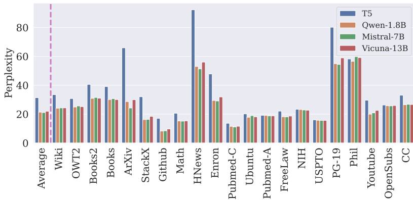
Figure 3: Importance of High Quality Paraphraser: Perplexity across all the Pile domains for WRAP on data generated by different LLMs. Results show that even small models like Qwen-1.8B can generate paraphrases of high quality. Though, a low quality rephraser like our fine-tuned T5-based model leads to significantly worse language modeling.
