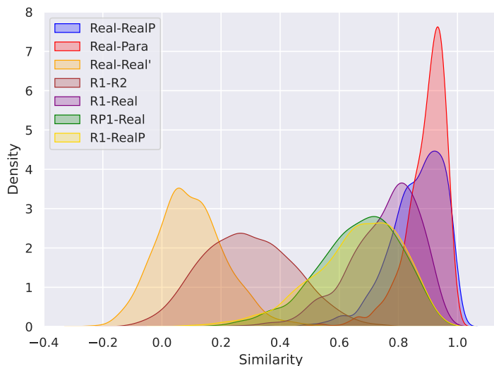
Figure 6: Cosine similarity medium synthetic MRPC rephrases
