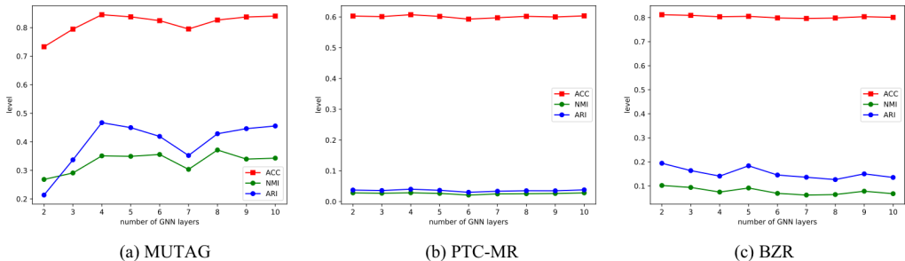
Figure 3: Sensitivity analysis of ACC, NMI and ARI regarding the number of GNN hidden layers on MUTAG, PTC-MR and BZR datasets
