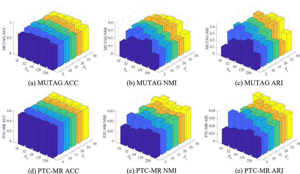
Figure 2: Sensitivity analysis of accuracy, NMI and ARI regarding the dimension d_h of GNN hidden layers and the embedding dimension d_z of clustering layer on MUTAG and PTC-MR datasets.
