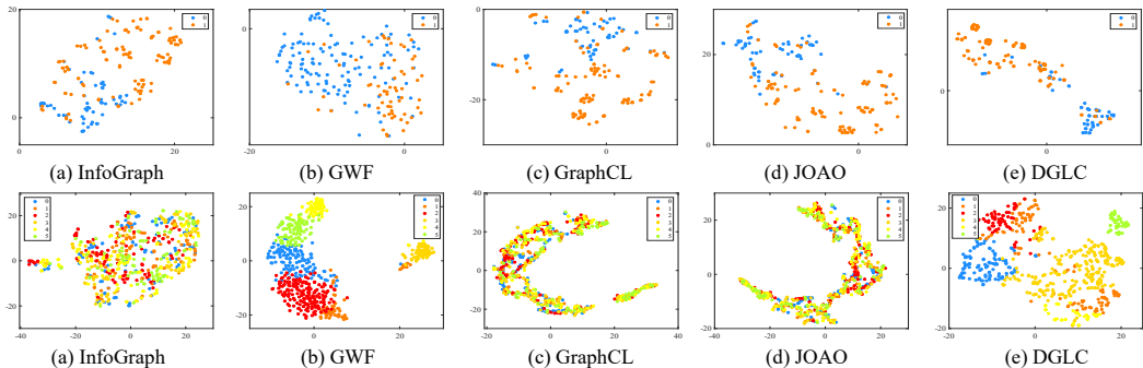
Figure 1: t-SNE visualization of the learned graph-level representations of our methods and other unsupervised graph representation learning methods. The first row is the visualization for MUTAG, while the second row is for ENZYMES.
