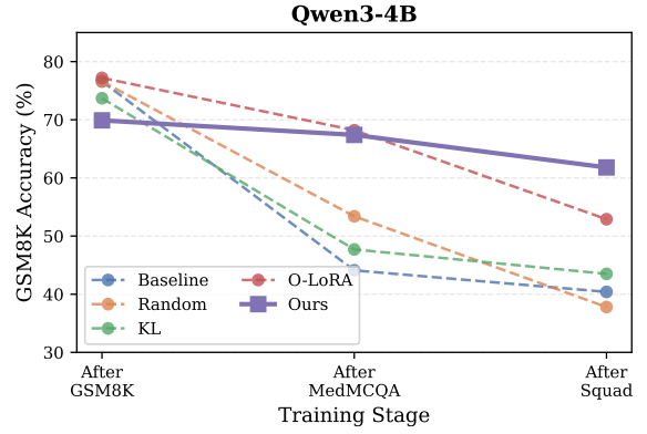
Figure 4: GSM8K trajectory on Qwen3. Moderate- G_i maintains gradual degradation while baselines exhibit catastrophic drops.
