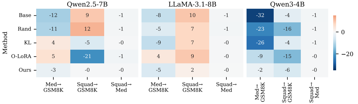
Figure 3: Task interference matrix. Negative values (blue) indicate interference; positive (red) indicates transfer. Moderate- G_i consistently minimizes cross-task interference.
