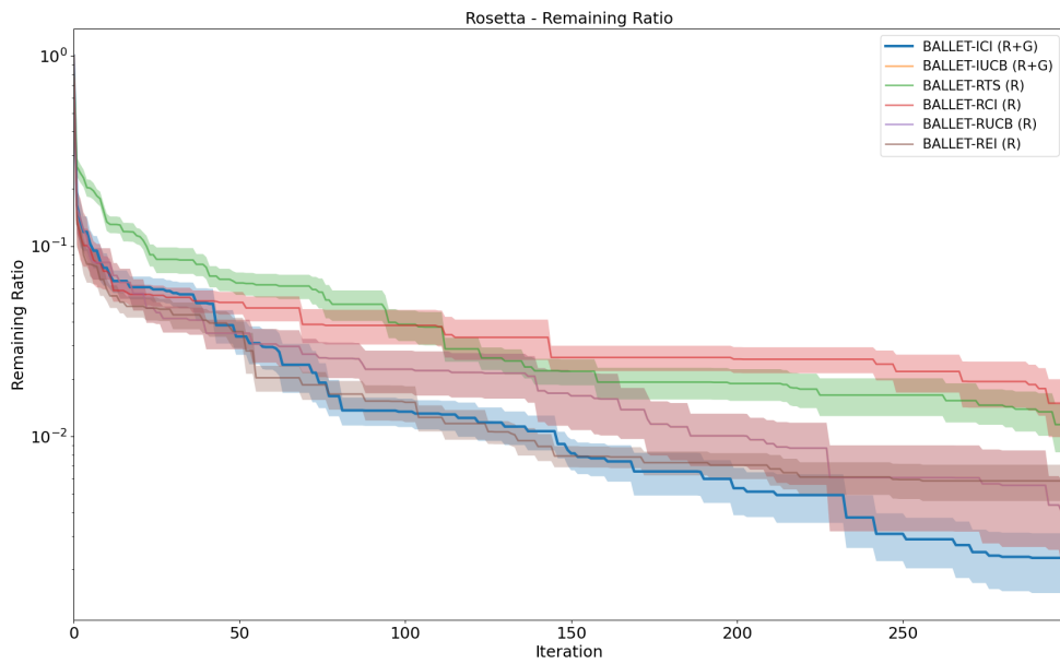
Figure 6: Simulation results on each task are shown here. The error bar demonstrates the standard error. The x-axis denotes the number of iterations, and the y-axis denotes the filtering ratio. The ratio for the 10 initial randomly picked warm-up datasets are clipped. (G), (R), and (R+G) means the global model only, the ROI model only, and the ROI model combined with the global model correspondingly.
