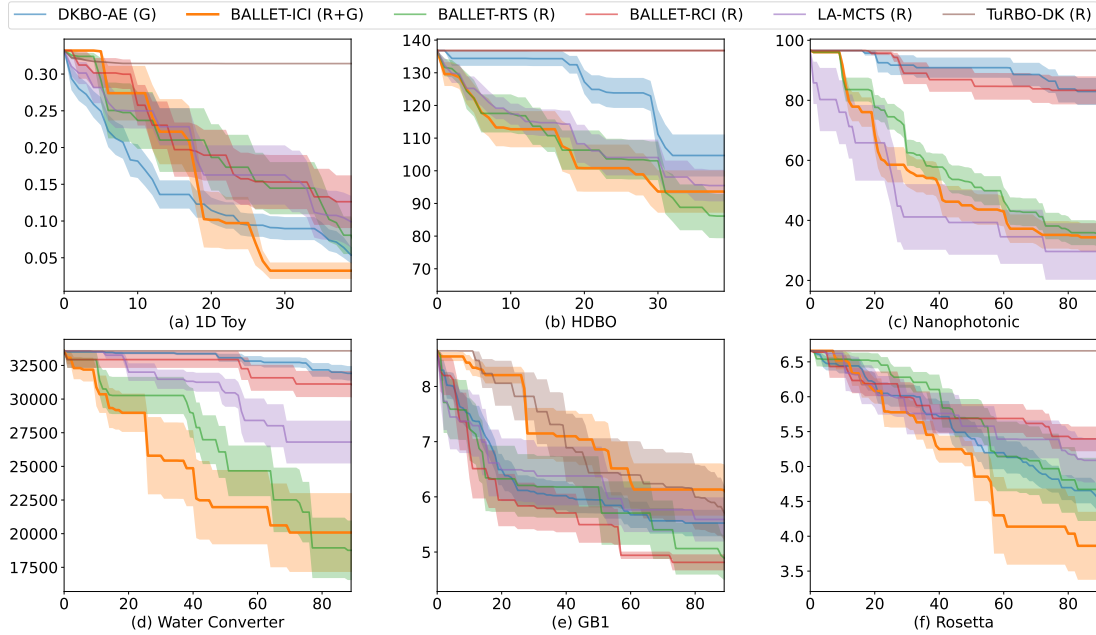
Figure 3: Simulation results. The results from each task are collected from at least 10 independent trials. The error bar demonstrates the standard error. The x-axis denotes the number of iterations, and the y-axis denotes the simple regret. The simple regrets for the 10 initial randomly picked warm-up datasets are clipped. (G), (R), and (R+G) means the global model only, the ROI model only, and the ROI model combined with the global model correspondingly.
