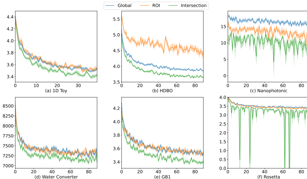
Figure 2: The confidence interval of f^* defined in Corollary 2. The results from each task are collected from at least 10 independent trials. The error bar demonstrates the standard error. As \beta varies on different iterations and different search space sizes, we fix \beta_t = 2 for comparable illustration. The x-axis denotes the number of iterations, and the y-axis denotes the width of the confidence interval.
