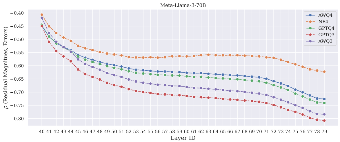
Figure 10: Correlations between the quantization errors \mathcal{E}(\mathcal{D}; \tilde{\theta}) and the residual magnitudes \mathbb{S}(\mathcal{D}; \theta; l) across the upper half layers of Llama3-70B. All methods show negative correlations in the last few layers.
