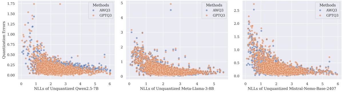
Figure 15: NLLs before quantization vs. quantization errors on different LLMs. Each dot represents a sample from FineWeb. In general, the low-frequency data (x-axis values \geq 4 ) have smaller errors. On the other hand, many samples that suffer from large quantization errors have small NLLs before quantization.
