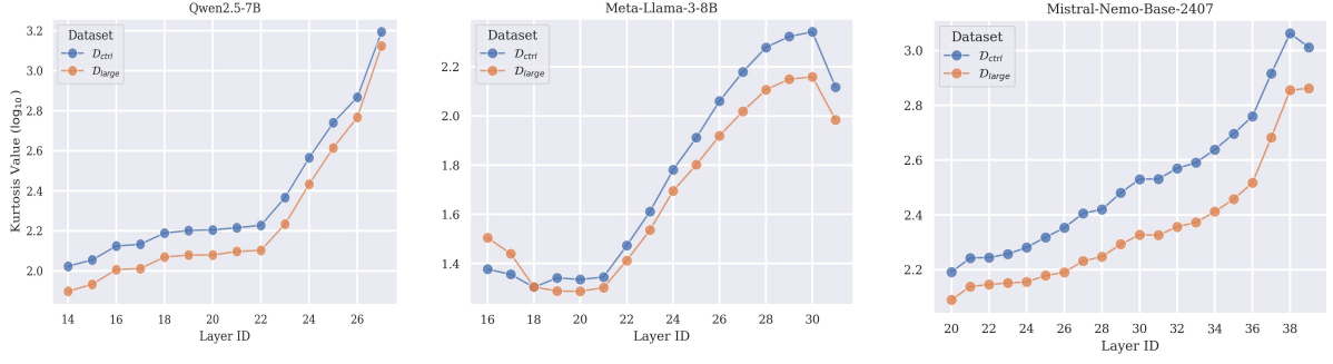
Figure 5: Kurtosis values of the residual states r^{(l)} from different full-precision LLMs (log scale). The large-error set \mathcal{D}_{\text{large}} shows lower kurtosis values than the control set \mathcal{D}_{\text{ctrl}} across layers, indicating that \mathcal{D}_{\text{large}} contains fewer or less extreme outliers in the residual states.
