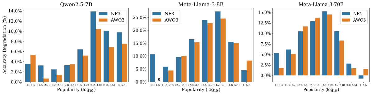
Figure 16: Accuracy degradation of different models on PopQA.
