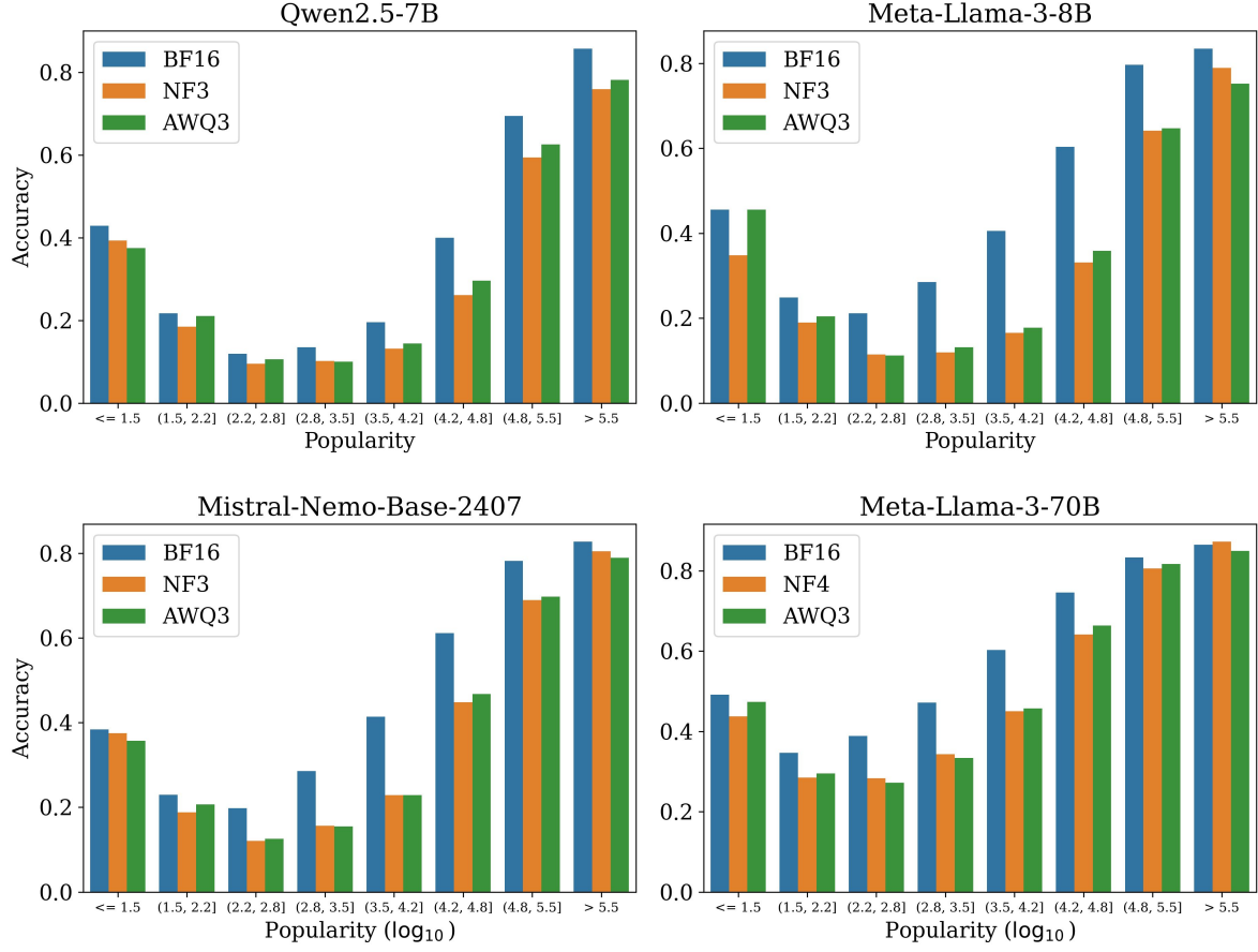
Figure 17: Absolute accuracies of different models on PopQA.
