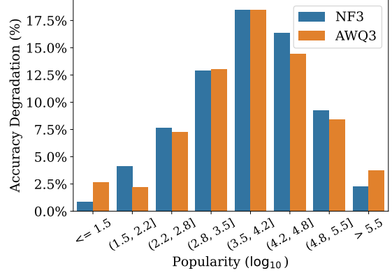
Figure 4: The accuracy degradation of PopQA under different levels of popularity after 3-bit quantization. Samples with log popularity between 2.8 and 4.8 show the greatest degradation.
