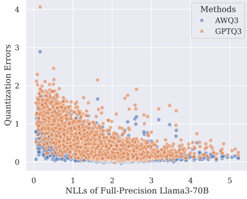
Figure 3: Long-tail samples with large NLLs on the full-precision Llama3-70B have small quantization errors. Each dot represents a FineWeb example. We quantize Llama3-70B with AWQ3 and GPTQ3 methods and compute their quantization errors with Eq. 4.
