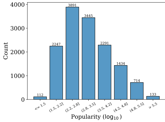
Figure 18: The histogram of the PopQA dataset. We partition the dataset into 8 buckets based on the sample popularity and ensure that each partition contains at least 100 samples.
