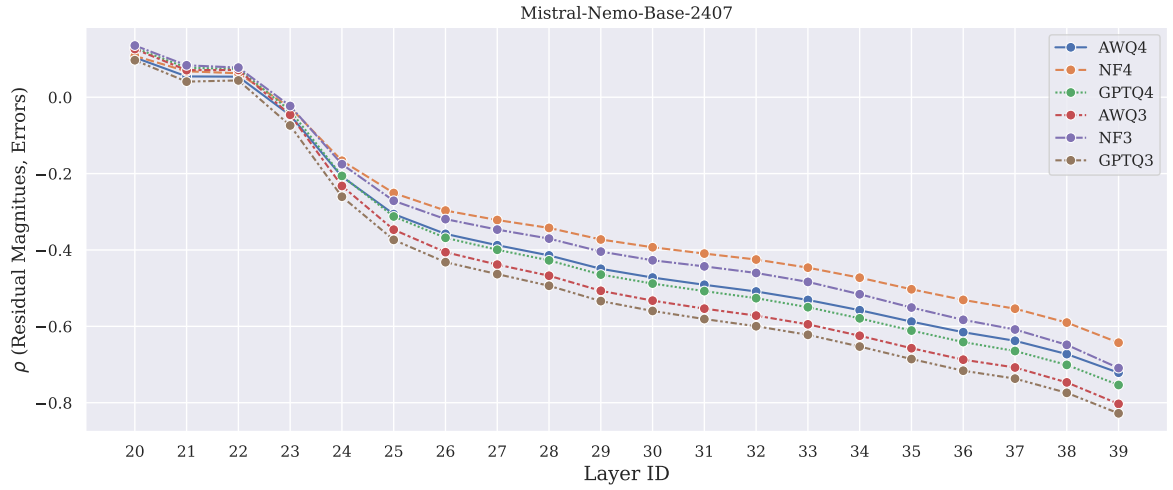
Figure 9: Correlations between the quantization errors \mathcal{E}(\mathcal{D}; \tilde{\theta}) and the residual magnitudes \mathbb{S}(\mathcal{D}; \theta; l) across the upper half layers of Mistral-12B. All methods show negative correlations in the last few layers.
