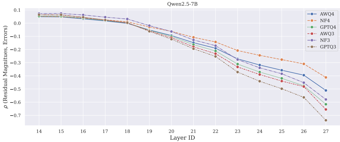
Figure 7: Correlations between the quantization errors \mathcal{E}(\mathcal{D}; \tilde{\theta}) and the residual magnitudes \mathbb{S}(\mathcal{D}; \theta; l) across the upper half layers of Qwen2.5-7B. All methods show negative correlations in the last few layers.
