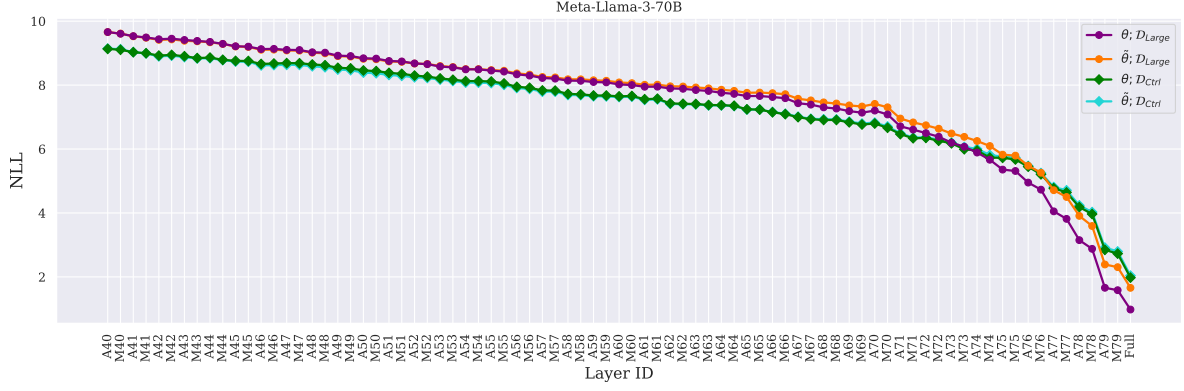
Figure 14: Early Exiting results on Llama3-8B. We decode z^{(l)} (A#) and r^{(l)} (M#) across layers.
