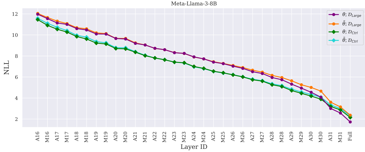
Figure 12: Early Exiting results on Llama3-8B. We decode the inputs to z^{(l)} (A#) and r^{(l)} (M#) across layers.
