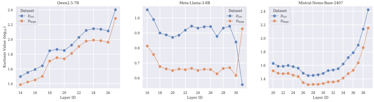
Figure 6: Kurtosis values of the post-RMSNorm hidden states h^{(l)} from different full-precision LLMs (log scale). The large-error set \mathcal{D}_{\text{large}} shows lower kurtosis values than the control set \mathcal{D}_{\text{ctrl}} , except for the last layer of Llama3-8B, indicating that overall \mathcal{D}_{\text{large}} contains fewer or less extreme outliers in the hidden states after RMSNorm. In addition, compared with Fig. 5 (before RMSNorm), the scale of the kurtosis values in this figure is much smaller (y-axis), implying that RMSNorm in the upper layers tends to suppress outliers.
