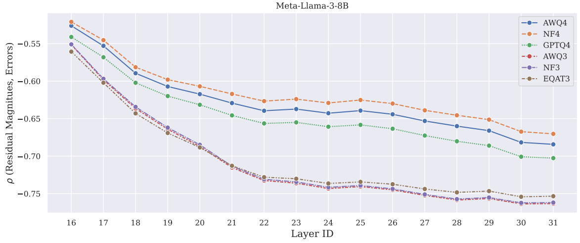
Figure 8: Correlations between the quantization errors \mathcal{E}(\mathcal{D}; \tilde{\theta}) and the residual magnitudes \mathbb{S}(\mathcal{D}; \theta; l) across the upper half layers of Llama3-8B. All methods show negative correlations in the last few layers.
