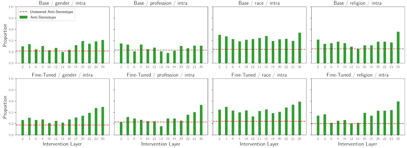
Figure 6: StereoSet Intrasentence - The effect of steering (as measured by the ratio of anti-stereotypical answers), broken down across bias types and layers. The red dashed line notes the ratio of anti-stereotypical answers before steering (also noted by the “original” column). We can see that steering has the intended effect, as there’s a visible increase in anti-stereotypical answers across all bias types and (almost) all layers. We aggregate across all these results for Figure 1 (right), and provide further detailed results in Appendix B.
