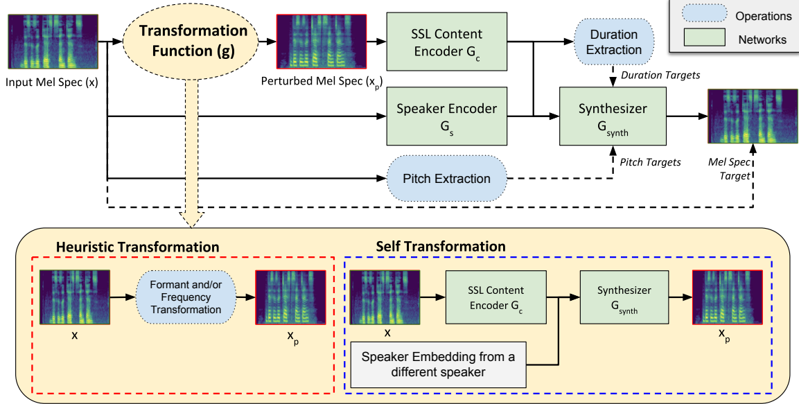
Figure 1: SelfVC Overview: The synthesizer G_{synth} is trained to reconstruct the mel-spectrogram from SSL-based content representation of a transformed audio and speaker embedding of the original audio. The transformation function is either a heuristic transform or a voice-converted audio generated using self-synthesis with a different speaker embedding.
