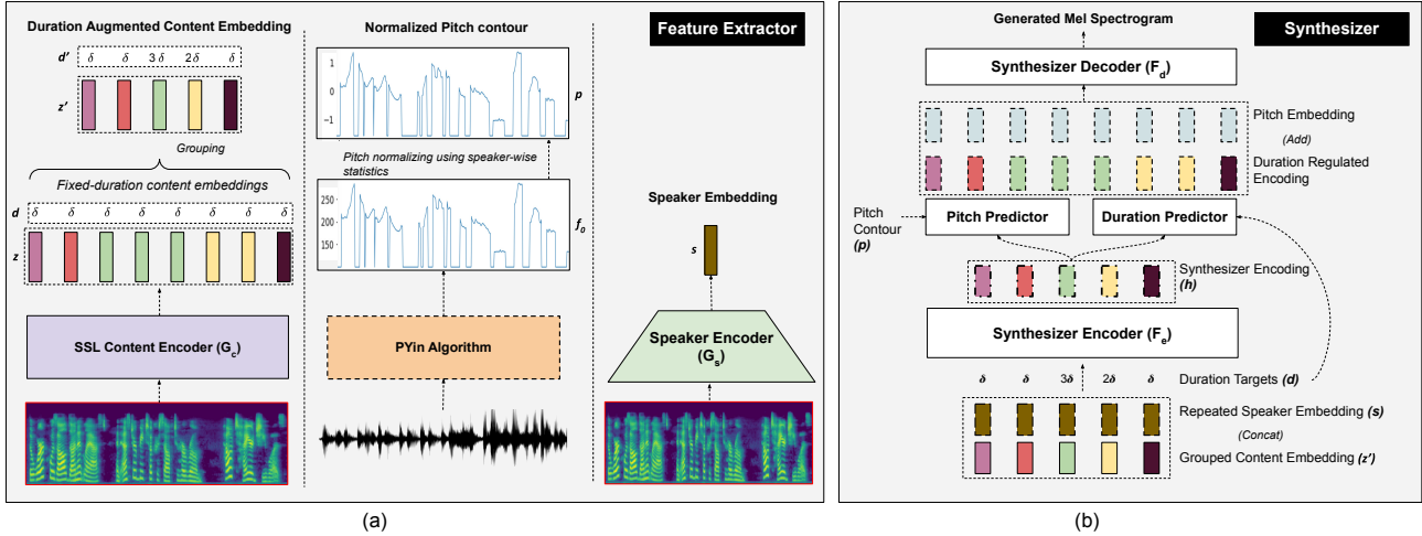
Figure 2: (a) Feature Extraction: The feature extractor derives the duration augmented content information from an SSL model, pitch contour using PYin algorithm and speaker embedding from a speaker verification model. (b) Mel Spectrogram Synthesizer: reconstructs the mel-spectrogram from the derived features.
