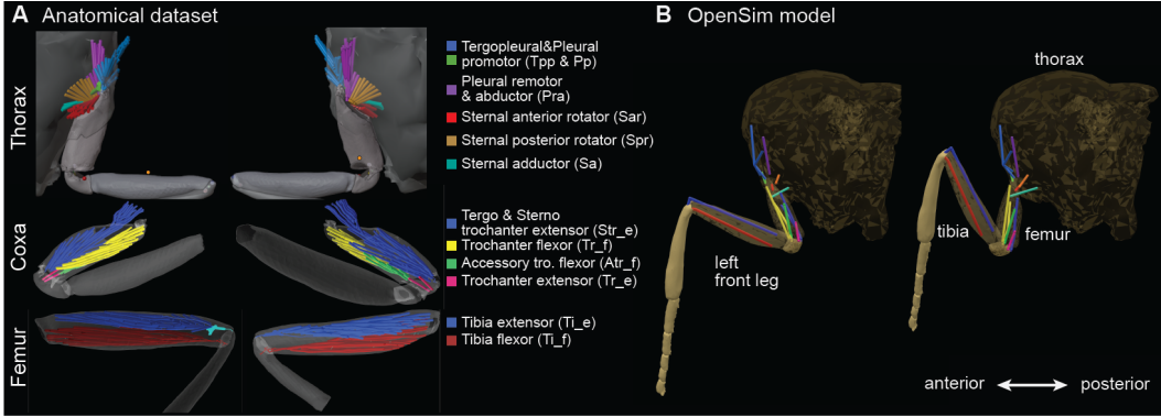
Figure 2: Front leg muscle reconstructions. (A) Muscles of the thorax, coxa, and femur were segmented from high-resolution X-ray scans (Kuan et al., 2020; Dinges et al., 2021) and visualized within a 3D mesh of the foreleg in Blender. Colors denote anatomically grouped muscles, including biarticular and joint-specific actuators. (B) Corresponding muscle-tendon units implemented in OpenSim preserve anatomical attachment points and fiber routing. Color coding is the same as in panel A.
