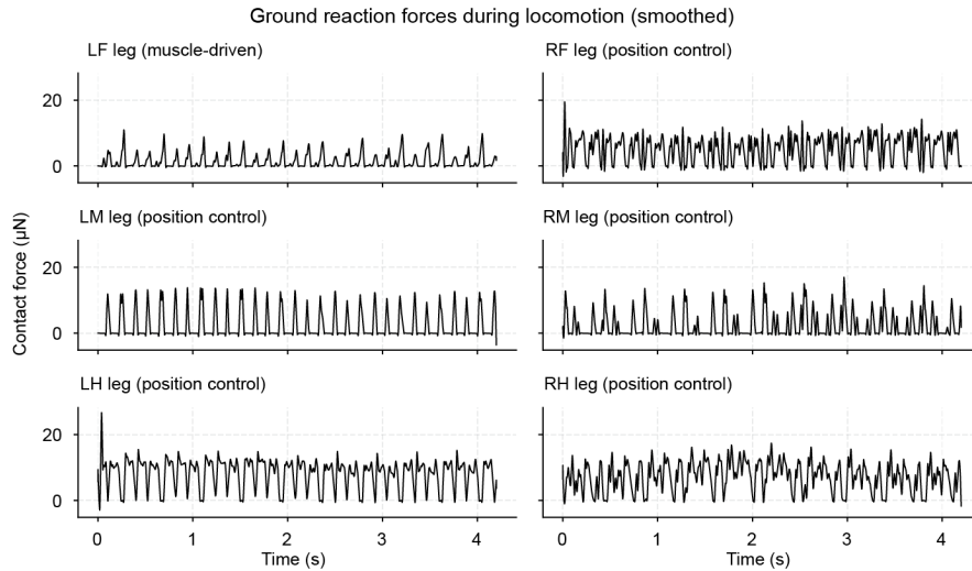
Figure S8: Ground reaction forces during contact-enabled locomotion. Smoothed ground reaction forces measured at each leg during locomotion with body-environment contacts enabled. The left foreleg (LF) is driven by the muscle activations produced by the trained policy (armature & stiffness & damping), while the remaining five legs (RF, LM, RM, LH, RH) are controlled via position controllers. Peaks in the force traces correspond to stance phases. Plotted values represent the norm of the ground reaction forces across the X, Y, and Z axes.
