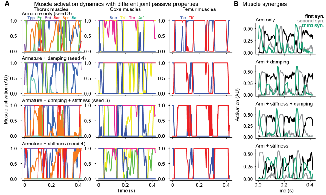
Figure S7: Muscle activation dynamics across passive joint conditions. (A) Simulated activation patterns of thorax (left), coxa (middle), and femur (right) muscles in PPO agents trained with varying passive joint properties: armature only (top), armature + damping (second row), armature + damping + stiffness (third row), and armature + stiffness (bottom). Each panel shows muscle activations from the best-performing seed for that condition. (B) Corresponding time courses of the first three extracted muscle synergies (black, gray, green), computed from the activation patterns shown in panel A.
