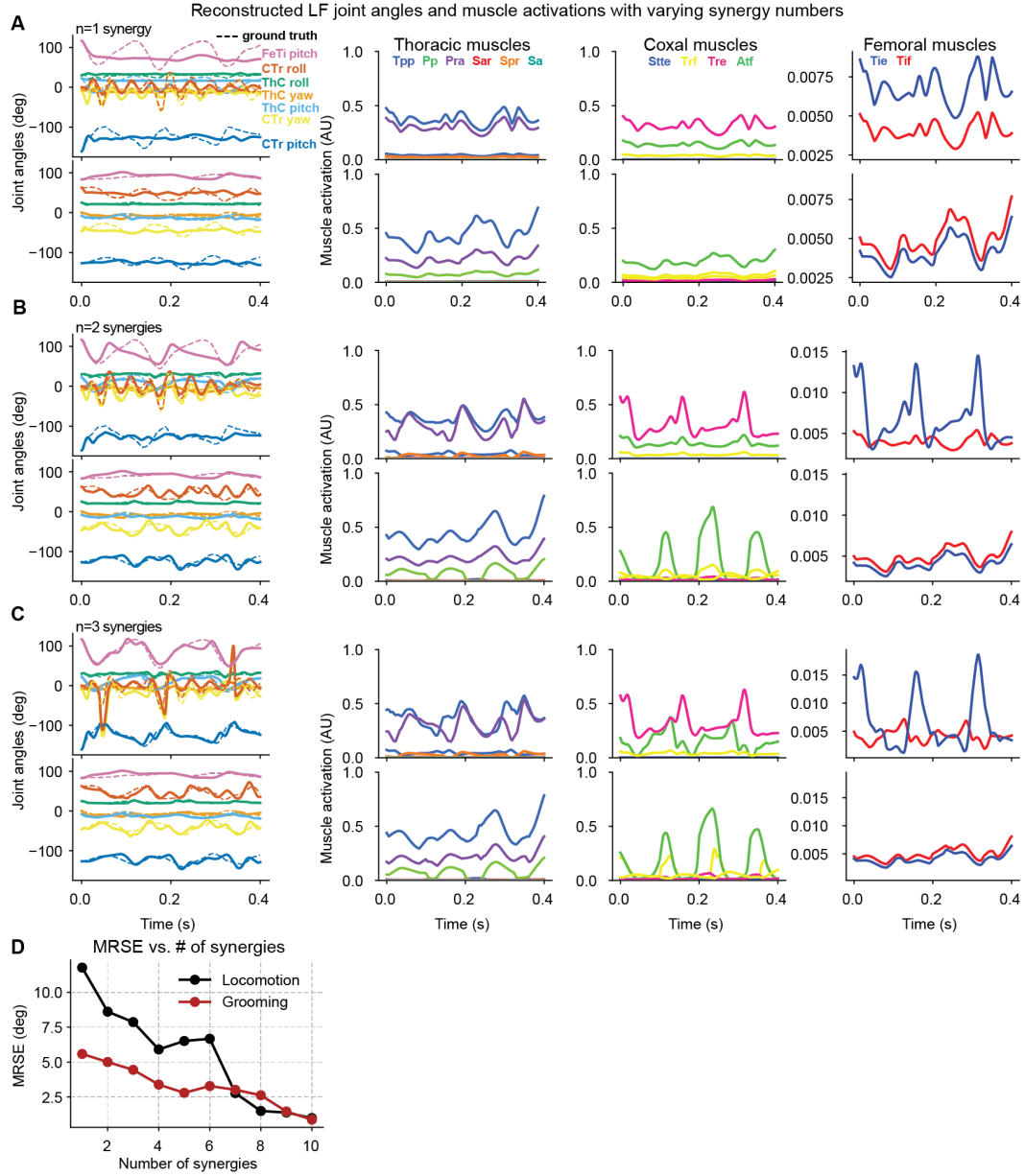
Figure S6: Reconstructed left foreleg (LF) joint kinematics and muscle activations using varying numbers of muscle synergies. (A–C) Reconstructed left foreleg joint angle trajectories (first column) and muscle activation dynamics for thoracic (second column), coxal (third column), and femoral (fourth column) muscles using (A) n=1 , (B) n=2 , and (C) n=3 synergies. Reconstructed joint angles are shown alongside ground-truth kinematics (dashed lines) for comparison. (D) Mean root-square error between reconstructed and ground-truth joint angles as a function of the number of synergies for grooming (red) and locomotion (black). Increasing the number of synergies improves reconstruction accuracy and yields more realistic muscle activation profiles across all muscle groups.
