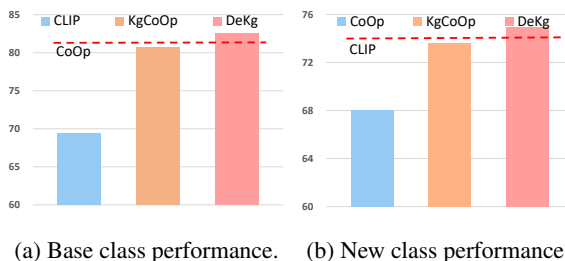
Figure 1: Performance comparison of DeKg with prompt tuning methods (CLIP/CoOp, KgCoOp (baseline method), and DeKg (Ours)) under base-to-new generalization setting. We measure average accuracy on the base classes (a) and new classes (b) over 11 datasets. The red dotted line indicates the performance of CoOp for base classes and the zero-shot CLIP for new classes.
