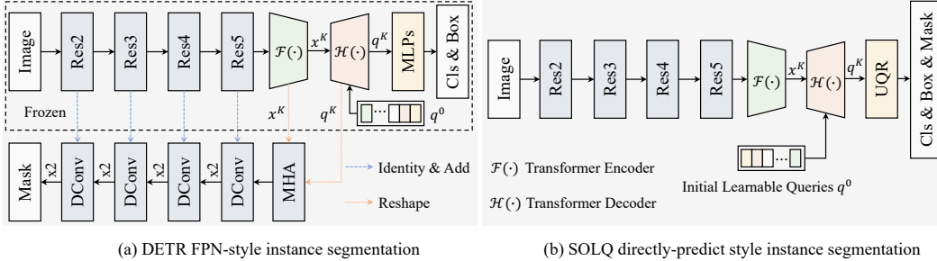
Figure 1: Architecture comparison between the naive DETR and the proposed SOLQ for instance segmentation. "Res2-Res5" are different stages of ResNet [50]. "DCConv" and "MHA" are deconvolution [51] layer and multi-head attention, respectively. "MLPs" means multi-layer perceptions and "UQR" denotes unified query representation, which is introduced in detail via Fig. 2. q^0 is initial learnable object queries. "Frozen" means that train object detector firstly, and then freeze weights of the object detector to train instance segmentation branch, separately.
