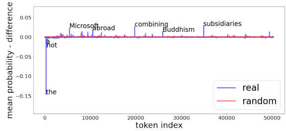
Figure 7: Differences in token probabilities before and after LN ln_1 from layer 15 of GPT-2 medium, according to the generations from section 3. The horizontal axis is the index of all the tokens in GPT-2 and the vertical shows if the token lost or gained probability from the process (negative or positive value). We annotate the tokens that are most affected.
