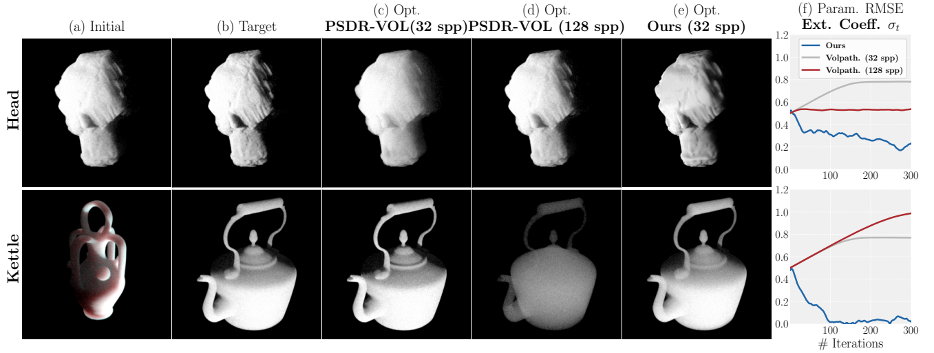
Figure 8: Comparison of shape-adaptive inverse rendering with PSDR-VOL [ZY21]. While the forward model of PSDR-VOL generates more physically accurate renderings, our results indicate that (c, e) the shape-adaptive BSSRDF achieves more accurate reconstructions of the extinction coefficient \sigma_t when evaluated at equivalent samples per pixel (spp). Notably, (e) the shape-adaptive BSSRDF demonstrates convergence at a low spp (32 spp), whereas (d) PSDR-VOL fails to converge even when utilizing a higher number of samples (128 spp).
