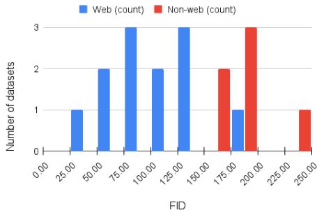
Figure 3: FID scores vs ImageNet for the datasets we study in this work (red), and the web-scraped datasets studied by Kornblith et al. (2019) (blue).
