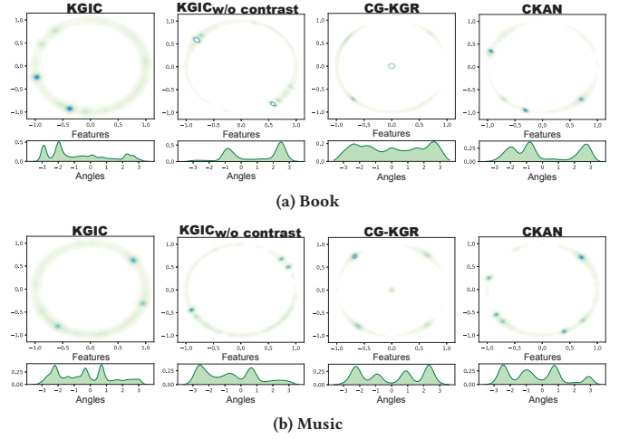
Figure 7: Visualization for the distribution of item embeddings.
