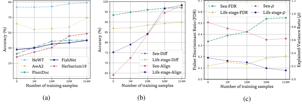
Figure 2: (a) The model performance on five downstream tasks under different scales of training data. (b) The model performance on differentiating and aligning different life stages and sexes. (c) The separation and orthogonality evaluation of models trained with different amounts of data.
