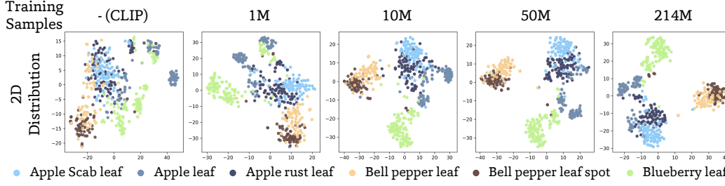
Figure 13: The t-SNE distribution of 6 classes from the PlantDoc dataset including three species and three different diseases. As the training data scales up, not only are the species better separated, but the intra-species variations also form clusters, making them easier to separate.
