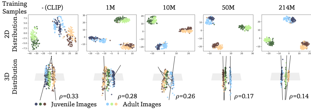
Figure 4: The embedding distribution of life stage variations under different scales of training data. The 2D distributions are obtained using t-SNE. For the 3D distributions, we first run SVD with the mean embedding of each species. The first two singular vectors are used to construct the gray plane that captures most inter-species differences. The embeddings are then projected into the 3D space with an additional orthogonal dimension. The straight lines point from the mean embedding of juvenile images to that of the adult images. As the training scales up, the intra-species variations are preserved in the subspace orthogonal to the inter-species differences. Orthogonality improves with data scale, as evidenced by the decreasing explained-variance ratio \rho .
