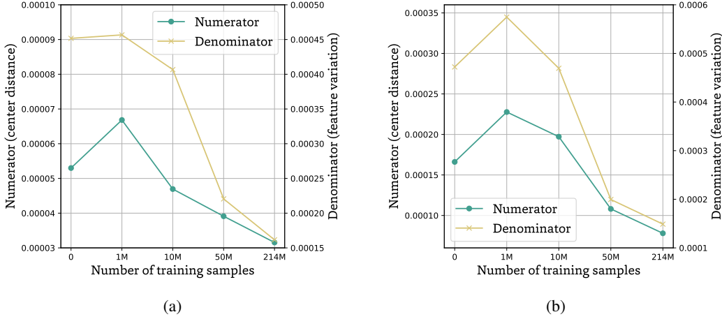
Figure 14: The decay curves for the numerator (difference between two class centers) and the denominator (feature variation) terms of the FDR metric along the increasing data scale. (a) The curves of life stage data. (b) The curves of sex data.
