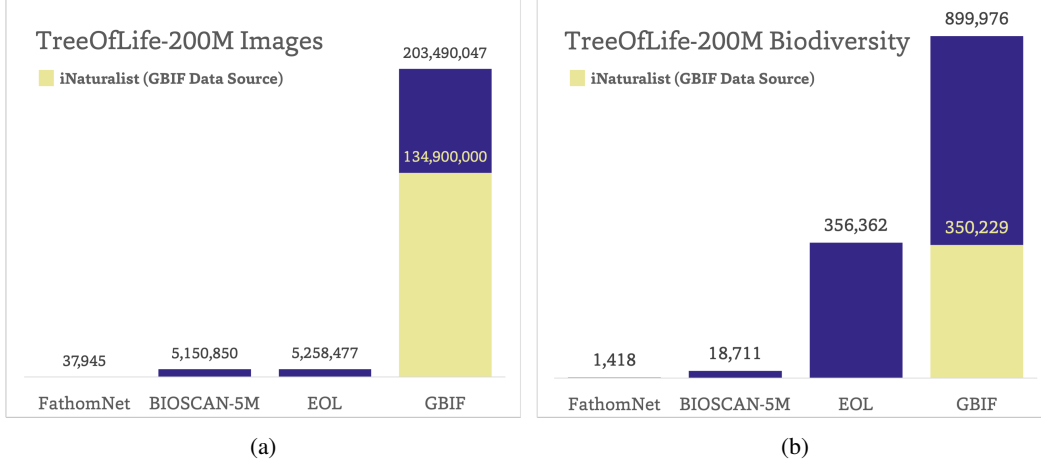
Figure 6: The number of images (a) and unique 7-rank taxa (b) by core data provider in TREEOFLIFE-200M. iNaturalist [59] is the largest GBIF data source (by image count) and the data provider used by BioTrove [14], so it is included here for reference.
