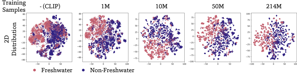
Figure 3: t-SNE embedding visualization of FishNet test set for models trained with different amounts of data. The leftmost plot is the original LAION-2B CLIP ViT-L/14. As the training data scales, freshwater fish become more distinct from saltwater fish and brackish fish, despite no explicit supervision, demonstrating that data scale contributes to emergent properties in model representations.
