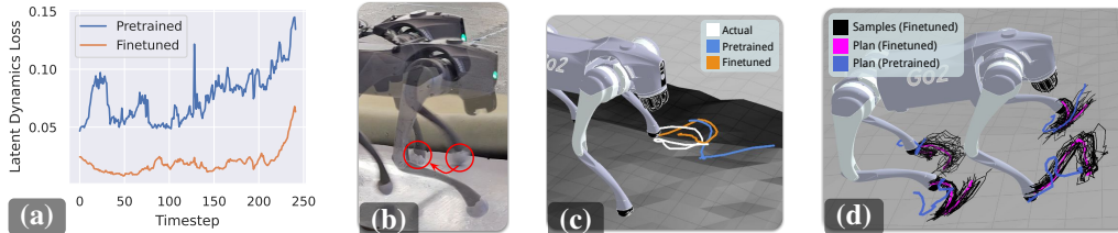
Figure 6: (a) Finetuning drastically lowers dynamics prediction loss during a quadruped PTFE trial. (b) Overlaid frames showing the front left foot slipping during a PTFE trial. (c) Foot-trajectory predictions from the world model at the same instant: the finetuned model correctly anticipates future slippage, while the pretrained model fails to do so. (d) Visualization of sampling-based planning. Candidate action sequences are evaluated with the world model to produce planned foot trajectories for each leg. Sampled trajectories are shown from the finetuned dynamics model, along with the resulting optimal plans under the finetuned and pretrained models. The finetuned model produces plans that account for real world dynamics mismatch, while the pretrained model generates qualitatively different trajectories.
