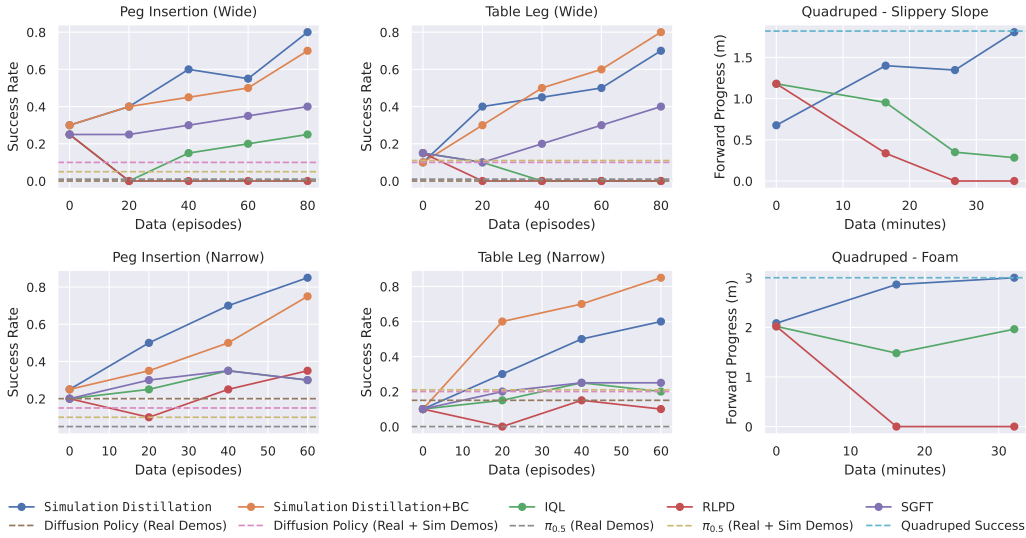
Figure 4: Real-world results. Success rate for two manipulation tasks, computed over 20 trials, and average forward progress for two quadruped locomotion tasks, averaged across all 15 trials (3 speeds, 5 trials each), as a function of real-world finetuning data. SimDist exhibits rapid and consistent improvement with limited data. In contrast, direct policy finetuning with the baselines shows limited or no improvement.
