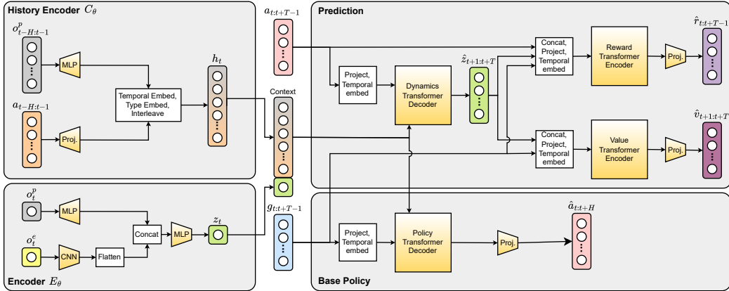
Figure 7: Detailed world model architecture for the quadruped.
