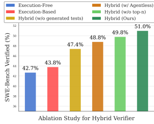
Figure 8: Ablation Study on Hybrid Verifier. We find three key insights: 1) While both execution-based and execution-free verifiers saturate around 42-43%, the hybrid approach yields significantly higher test-time gains (51%). 2) Regression tests alone are insufficient for hybrid scaling — achieving only 47.4% aggregation performance. 3) Agentic vs Agentless: training a specialized testing agent is important improving the performance from 48.8% to 51%.
