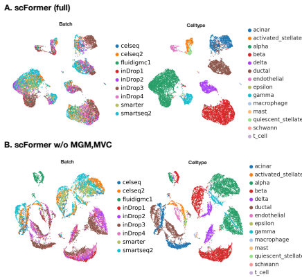
Figure 3: UMAP Visualizations.
