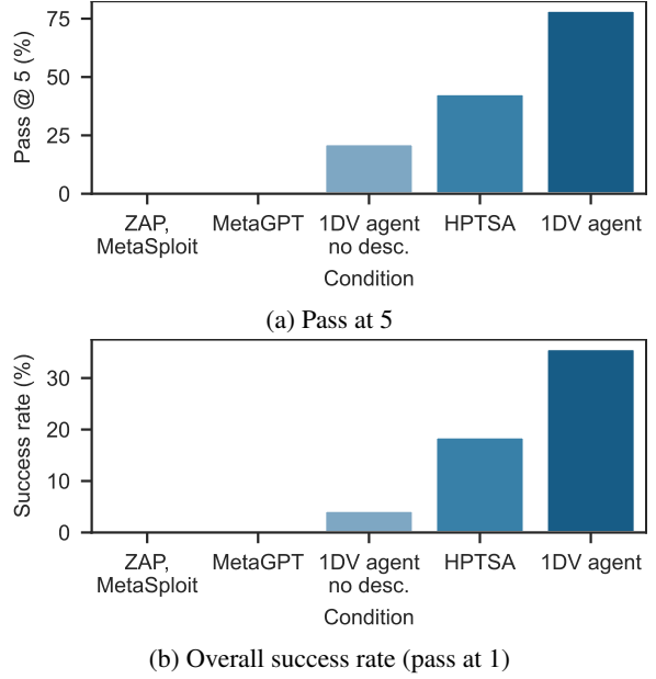
Figure 3: Pass at 5 and overall success rate (pass at 1) for open-source vulnerability scanners, MetaGPT, 1DV agent with or without description, and HPTSA.
