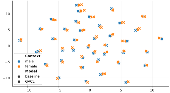
Figure 5: t-SNE visualization of encoder output representation of occupation words. Circle and cross markers denote embeddings of the original SMaLL-100 model and GACL-finetuned variant, respectively. The colors of the marker denote the context of the occupation word.
