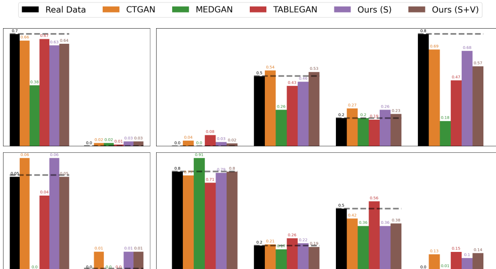
Figure 3: Histogram chart of subgroups for our synthetic variables V1 (top left), V2 (bottom left), V3 (top right) and V4 (bottom right) for the Child dataset. The real data values are shown in black. The plot shows which models suppress subgroups in their generated data. Suppressing features could have consequences for the synthetic dataset’s general performance, fairness and semantic integrity.)
