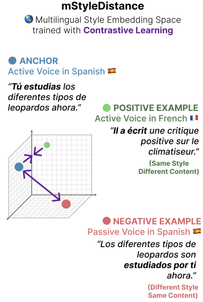
Figure 1: MSTYLEDISTANCE is trained using contrastive learning from synthetic positive and negative examples of ~40 style features in 9 languages to form both multilingual and cross-lingual training triplets.
