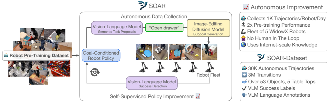
Figure 1: We introduce SOAR, an approach to autonomously improve instruction following policies by leveraging foundation models for large-scale autonomous data collection and self-improvement with no human in the loop. SOAR imports Internet-scale knowledge from pre-trained Vision-Language Models and image-editing Diffusion Models to guide autonomous data collection, and enables policy-improvement with a self-supervised objective on the autonomous data. We make available the 30.5K autonomous trajectories collected with SOAR in SOAR-dataset.
