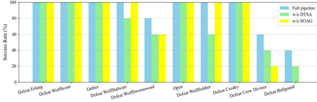
Figure 4: Ablation study.
