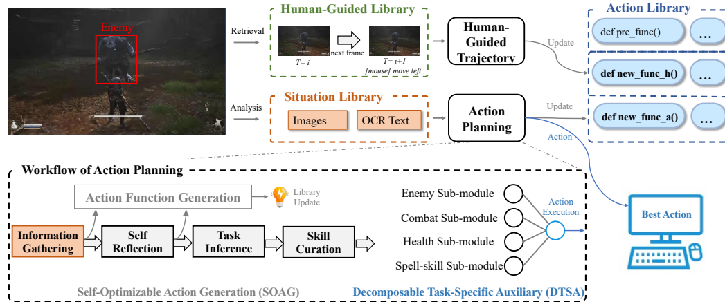
Figure 1: Pipeline of VARP. We propose a novel framework named the VARP agent, which directly takes game screenshots as input and generates keyboard and mouse operations to play the ARPG.
