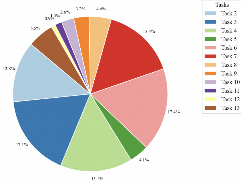
Figure 7: Dataset composition.
