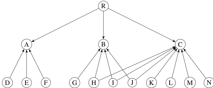
Figure 3: An example of a Bayesian network where greedily choosing to reverse edges when marginalizing out node R is not optimal.
